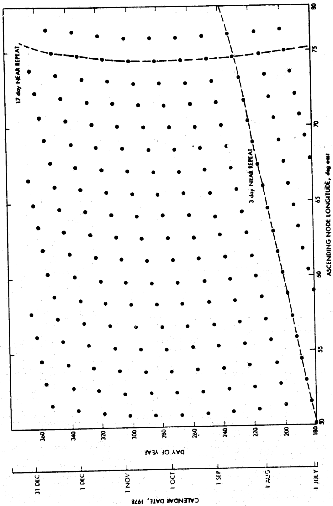
Figure 5-6. Seasat Launch Orbit Ascending Node Pattern
