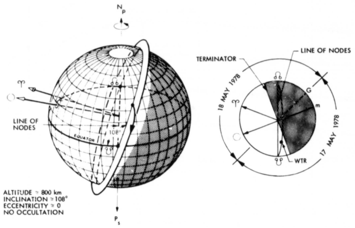
Figure 4-3. Seasat Orbit Geometry for 18 May 1978 Launch
