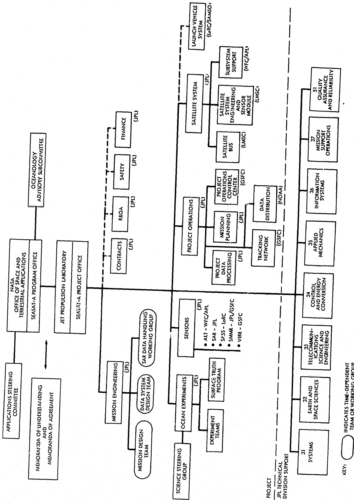
Figure 3-2. Seasat Project Relationships
