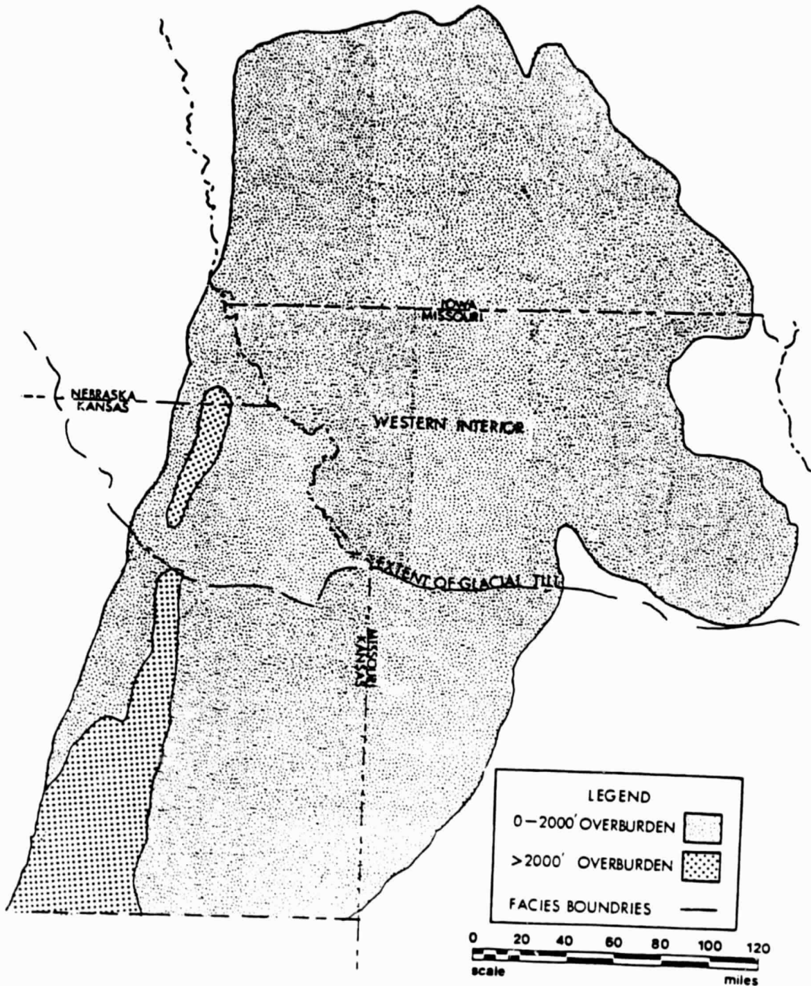
Figure 11. Location of Area of Coal Resource Estimation for the Western Interior Basin in the Carboniferous Interior Province (See Table A-21 for resources.)
