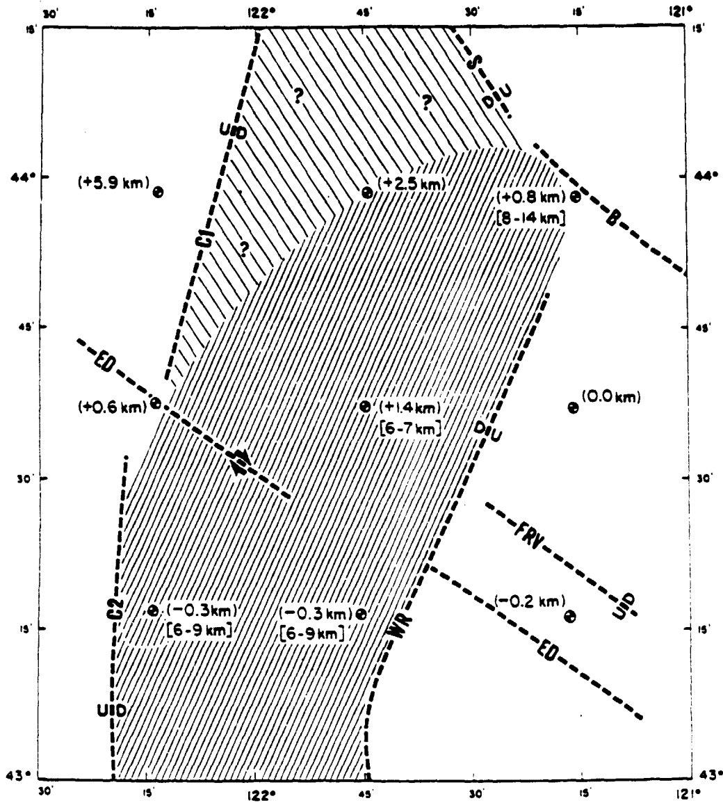
TECTONIC MAP
