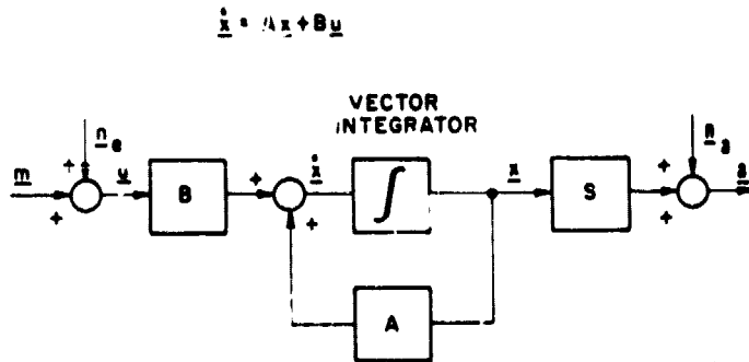
Fig. 1. Definitions: x = body "actual state" vector u = forcing vector: = n_e + m m = motor outflow vector (from CNS) a = polysensory afference vector (to CNS) n_e = external disturbance "noise" vector n_s = sense organ output "noise" vector
