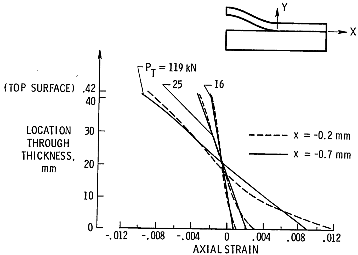
Fig. 4— Variation of axial strain through thickness of buckled region ( 2a = 25 \text{ mm} ), nonlinear analysis.
