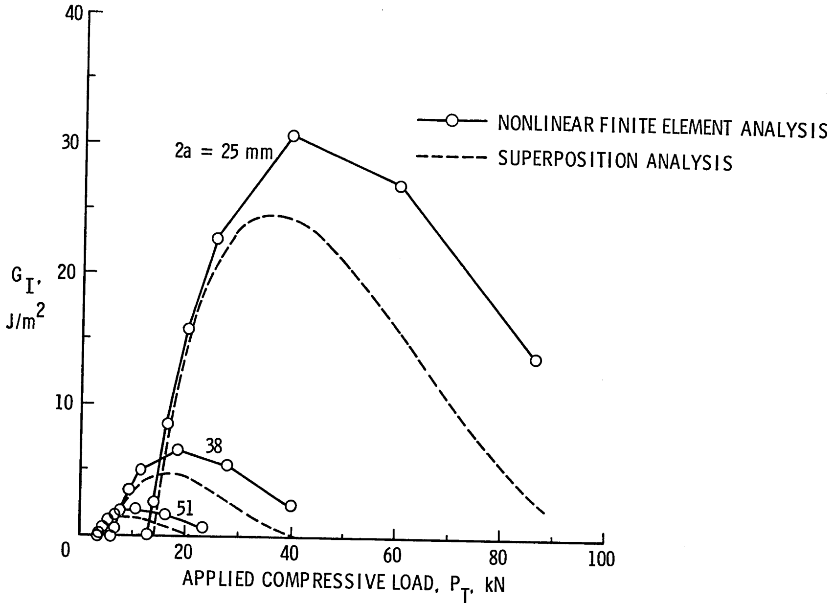
Fig. 6— Evaluation of approximate superposition analysis ( (P_C - P_D) and M from strength of materials analysis).
