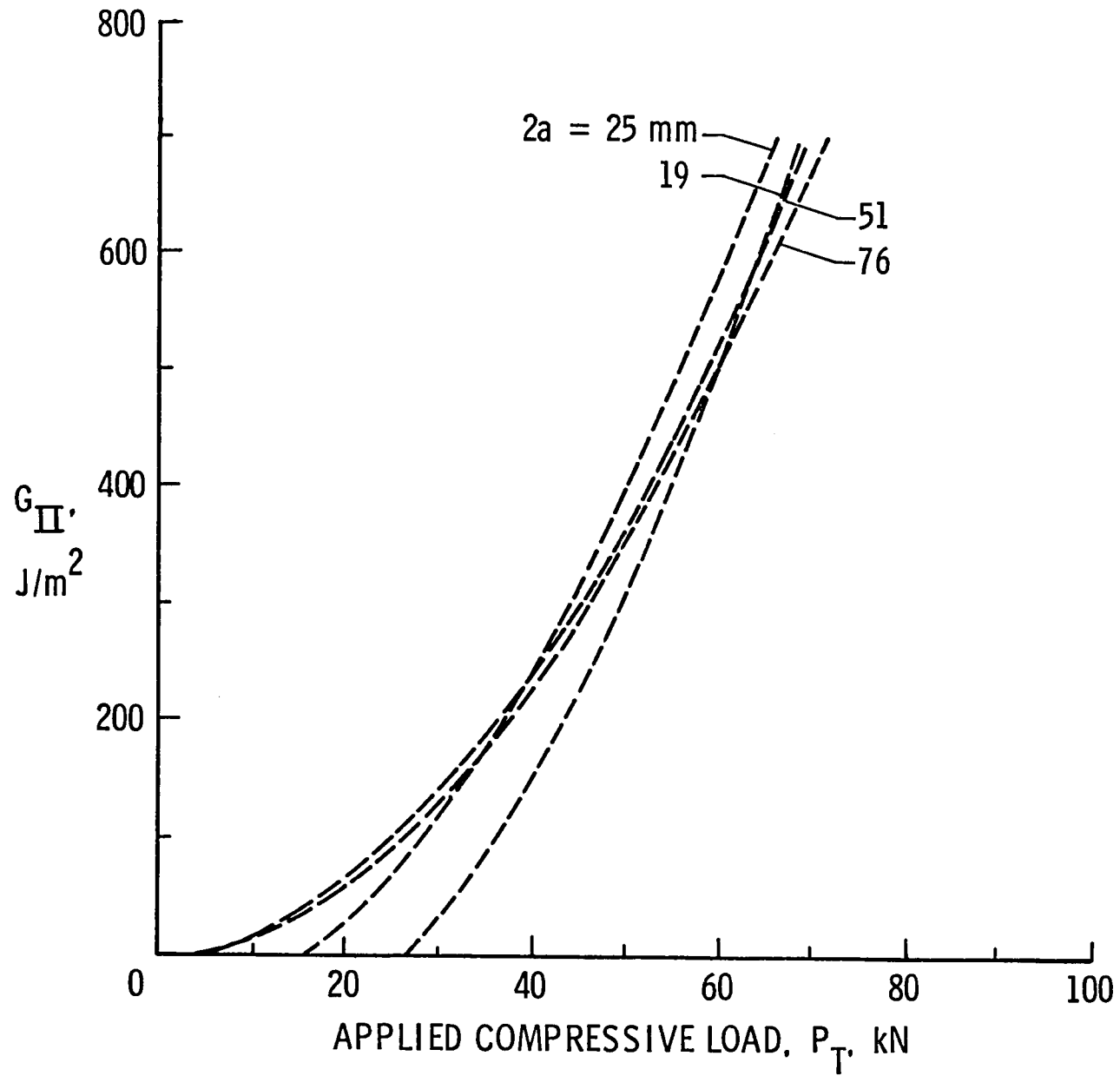
Fig. 14— Effect of applied compressive load on G_{II} ( 2a = 25 mm ).
