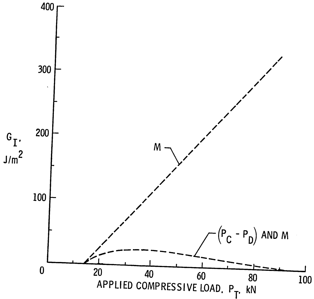
Fig. 8— Effect of (P_C - P_D) and M on G_I ( 2a = 25 mm).
