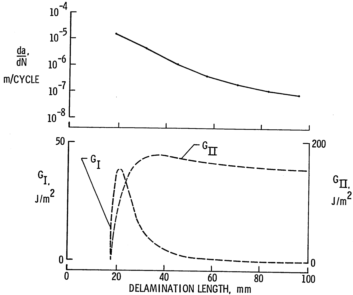
Fig. 16— Comparison of G_I , G_{II} , and delamination growth rate for maximum fatigue load of 33 kN.
