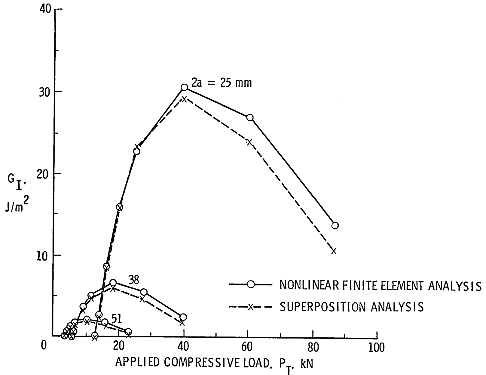
Fig. 5— Evaluation of approximate superposition analysis ( (P_C - P_D) and M from nonlinear finite element analysis).
