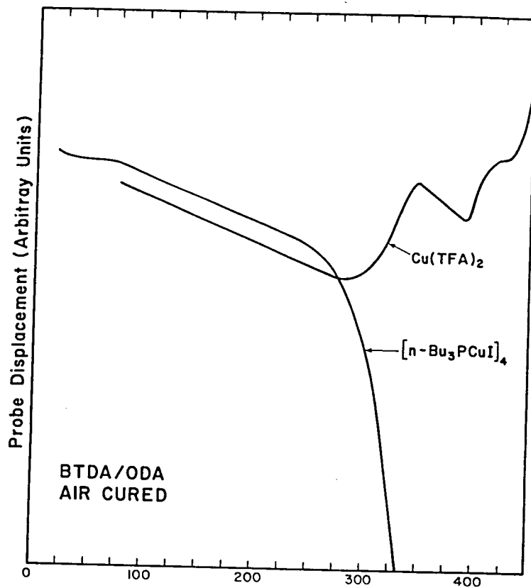
Figure 1. Plot of Thermomechanical Analysis of BTDA-ODA Film (air-cured) Doped with [(n\text{-Bu}_3\text{PCuI})_4] and \text{Cu}(\text{TFA})_2 .
