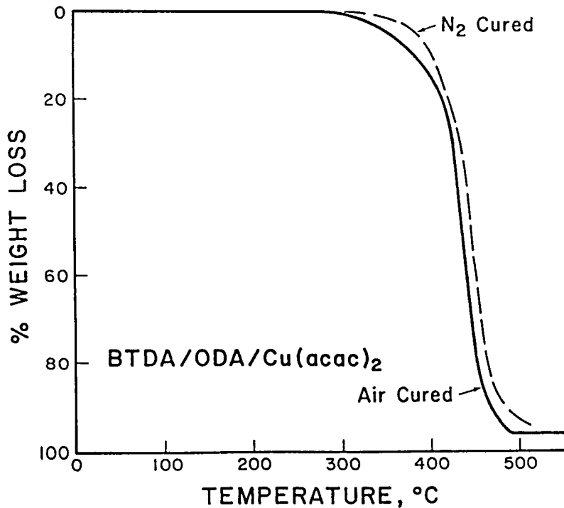
Figure 4. Plot of Thermal Gravimetric Analysis of BTDA-ODA-Cu(acac) 2 Film Cured in Air and N 2 .
