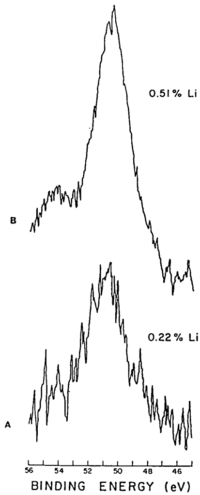
Figure 10. Concentration Dependence of Lithium 1s Photopeak.
