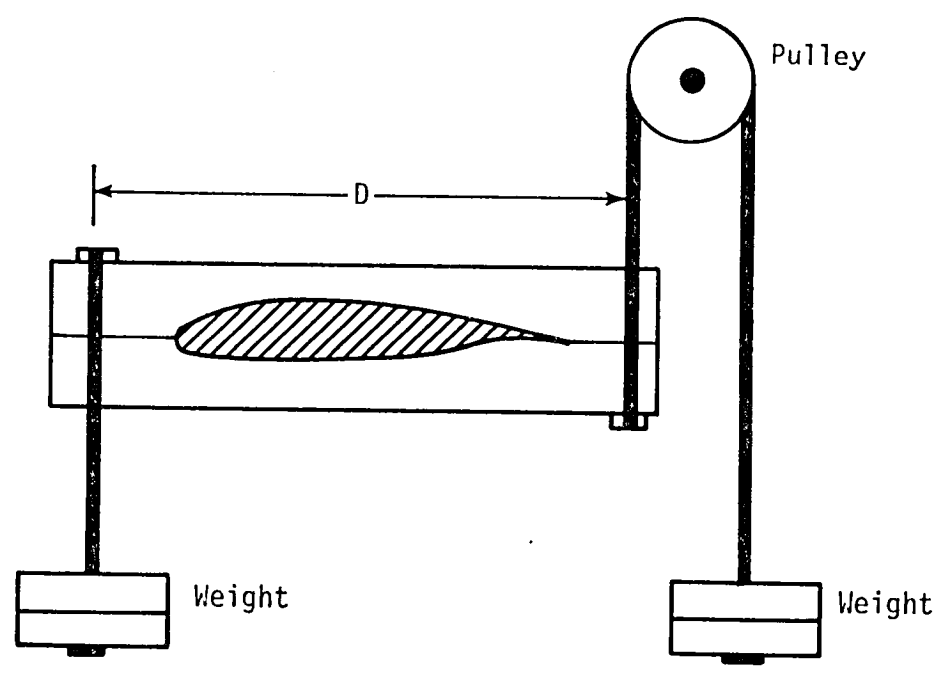
Figure 4.- A typical loading fixture for applying moments.
