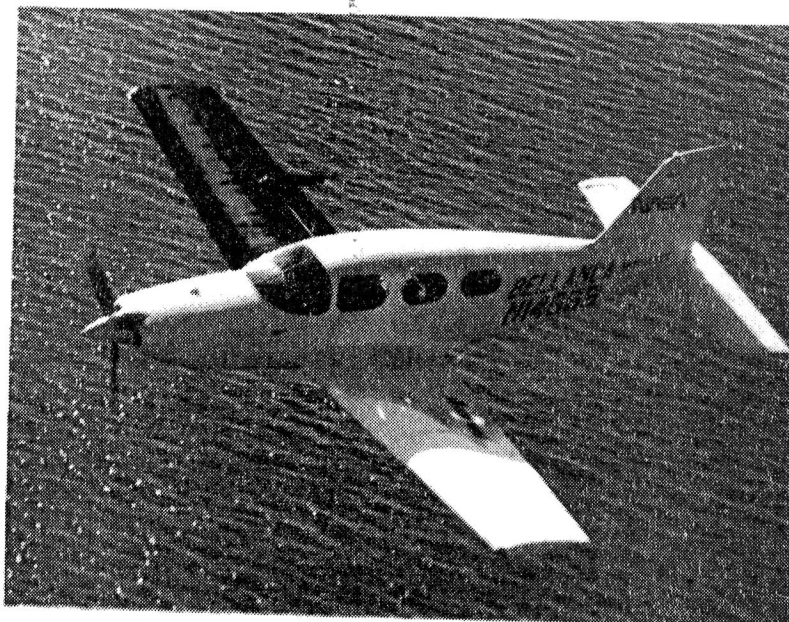
Figure 35.- Experimental aircraft for conducting laminar flow studies.
