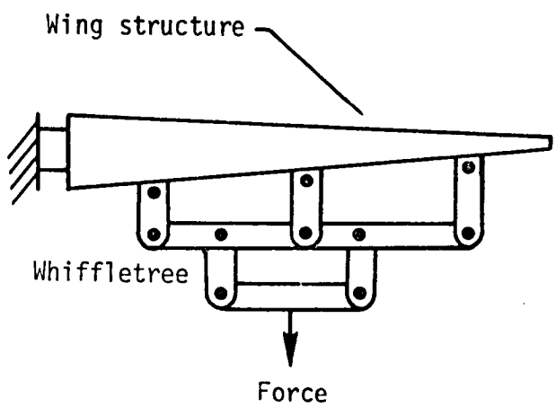
(b) Whiffletree
