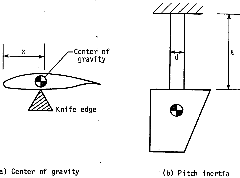
Figure 28.- Measurement of mass properties of wing.
