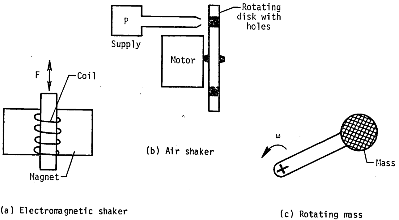
Figure 30.- Typical devices for exciting a structure.
