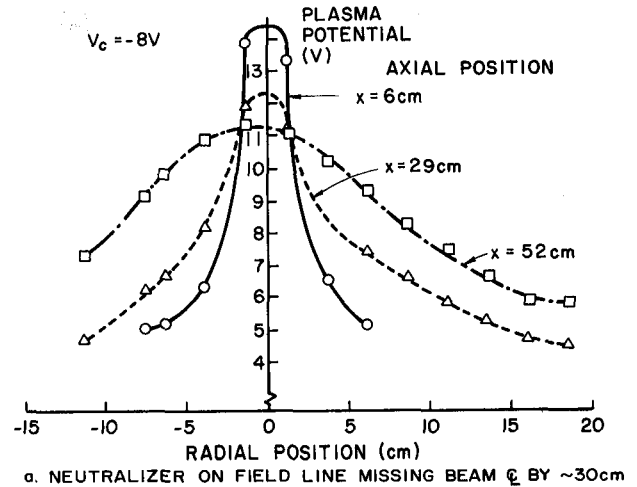
a. NEUTRALIZER ON FIELD LINE MISSING BEAM \phi BY \sim 30 cm
