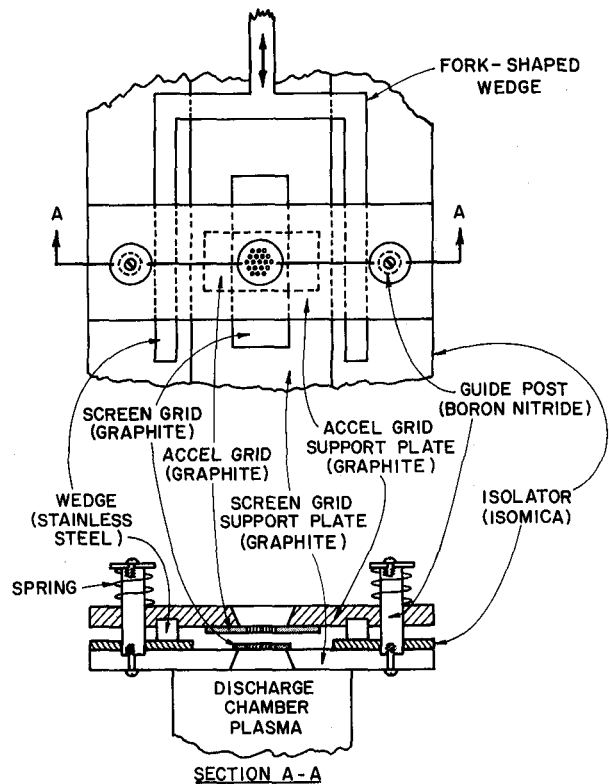
Fig. 2 Variable Grid Spacing Apparatus
