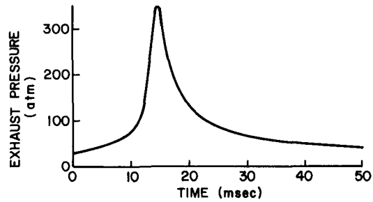
e. Projectile Base Pressure Profile
