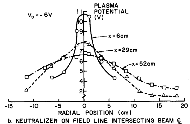
b. NEUTRALIZER ON FIELD LINE INTERSECTING BEAM \phi
