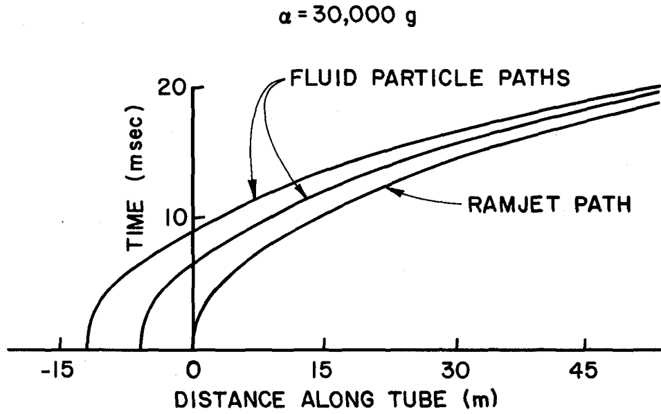
Fig. 14 Uniform Acceleration: Time vs. Distance
