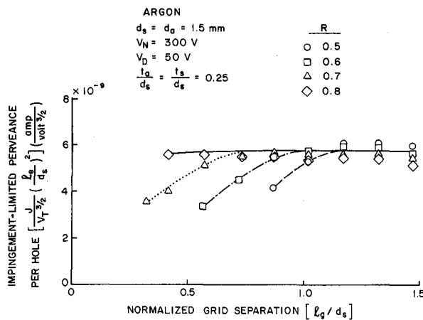
Fig. 9 Effect of Net-to-Total Acceleration Voltage Ratio on Ion Extraction Performance for 1.5 mm Diameter Grid Apertures
