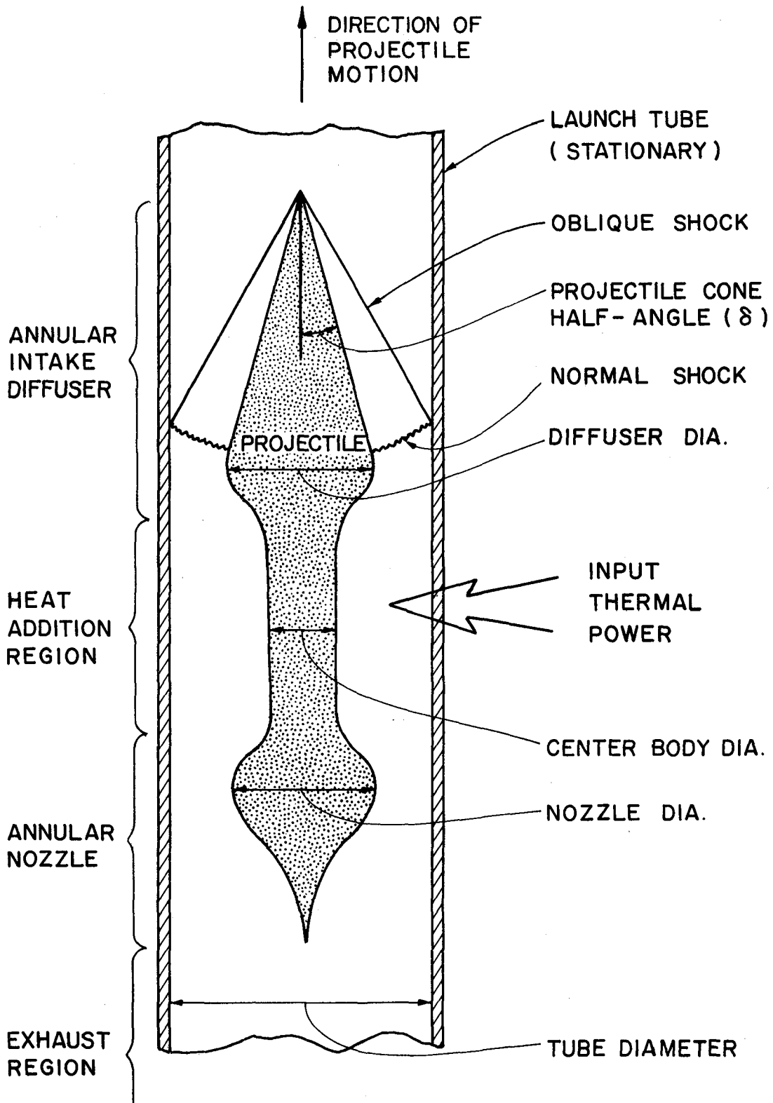
Fig. 12 Electrothermal Ramjet Schematic
