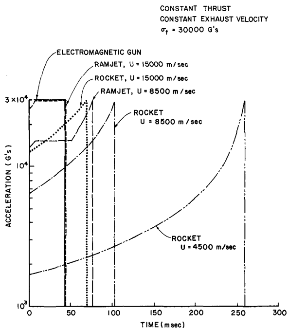
Fig. 5. Acceleration Profile Comparison
