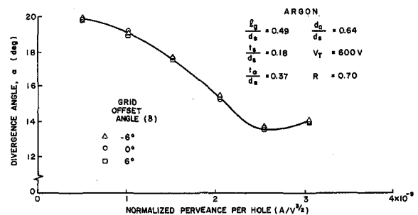
Fig. 6. Effect of Grid Offset on Beamlet Divergence.
