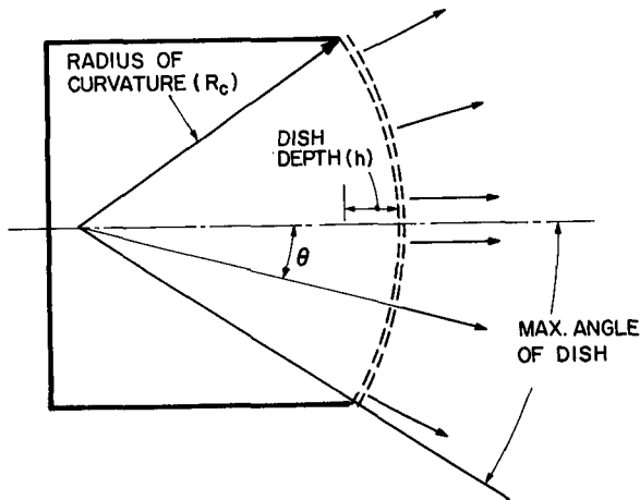
Fig. 20. Dished Grid Geometry.
