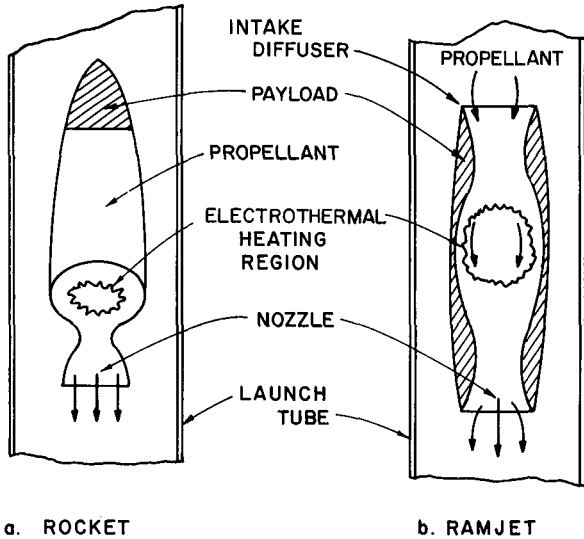
Fig. 1. Electrothermal Thruster Concepts
