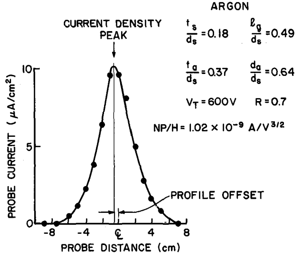
a. BEAM CURRENT DENSITY PROFILE
