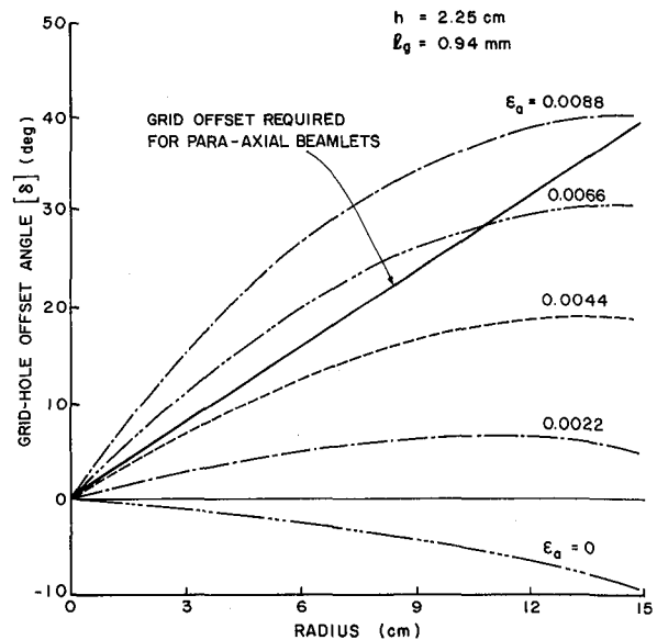
Fig. 22. Dished Grid Offset Angles for Varying Accelerator Grid Compensation, h = 2.25 .
