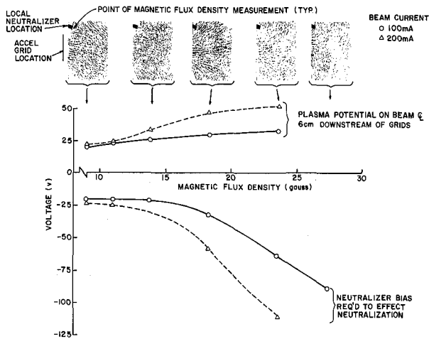
Fig. 13 Effect of Magnetic Field at Local Neutralizer on Beam and Neutralizer Potentials
