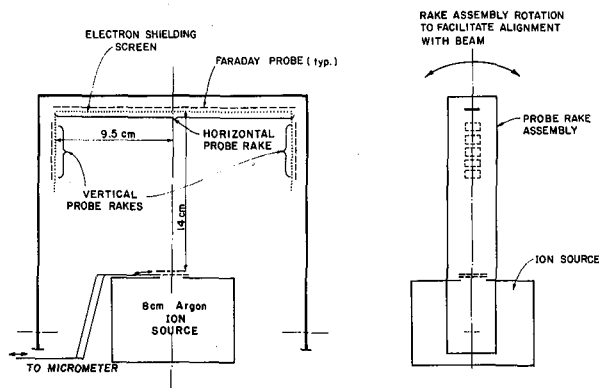
Fig. 2. Deflecting Beamlet Test Apparatus.
