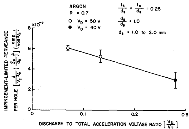
Fig. 8 Effect of Discharge-to-Total Acceleration Voltage Ratio on Ion Extraction Performance
