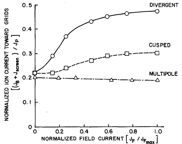
Fig. 5 Normalized Ion Current Directed Toward Grids vs. Field Current.
