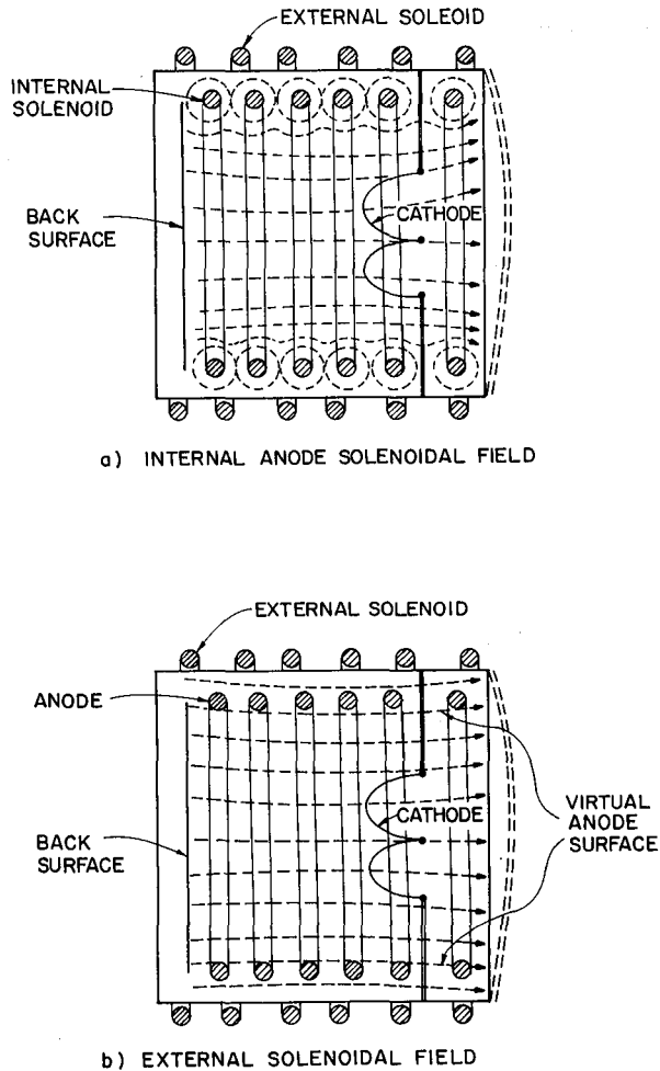
Fig. 8 Axial Magnetic Field Thruster Configurations.
