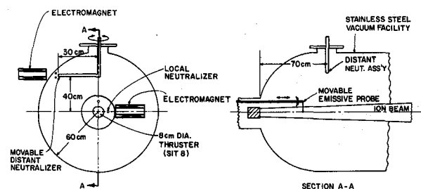
Fig. 1 Neutralization Test Apparatus
