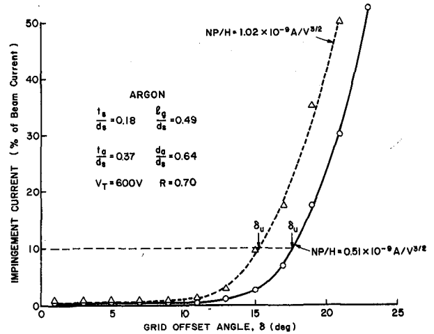
Fig. 5. Effect of Grid Offset on Impingement Current.
