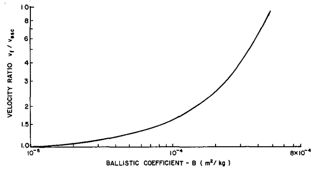
Fig. 3. Velocity Loss Through Atmospheric Drag
