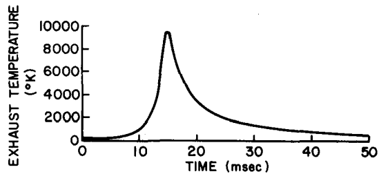
f. Exhaust Temperature Profile
