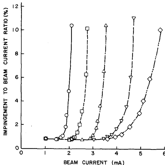
Fig. 3 Effect of Grid Separation on Impingement Curves - Nineteen Hole, Two-Grid Systems
