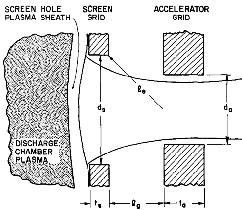
a) GRID GEOMETRY
