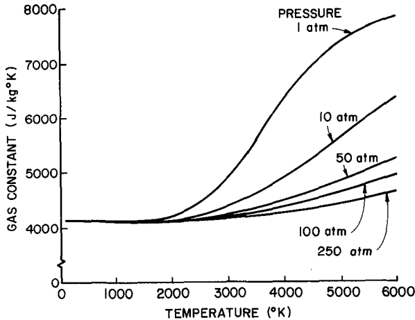
Fig. 10. Gas Constant for Equilibrium Hydrogen
