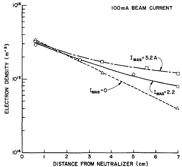
Fig. 9 Electron Density Profile for Axial Magnetic Field Case
