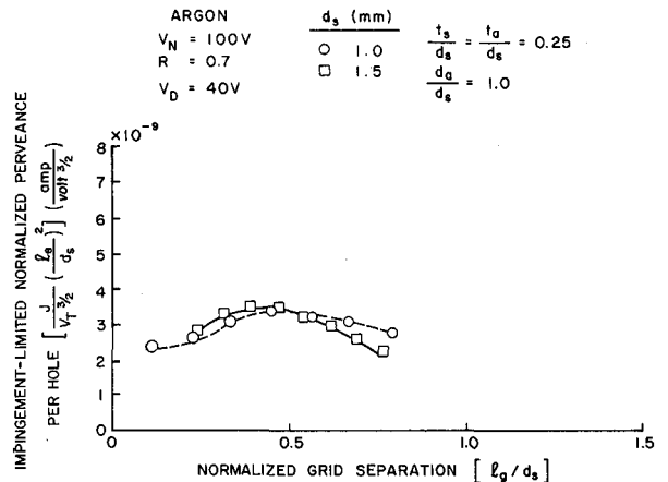
Fig. 6 Effect of Aperture Diameter on Two-Grid System Ion Extraction Performance for a Net Accelerating Voltage of 100 V
