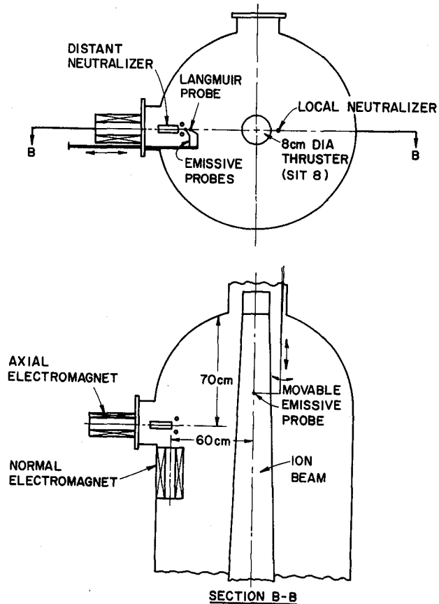
Fig. 2 Neutralization Test Apparatus
