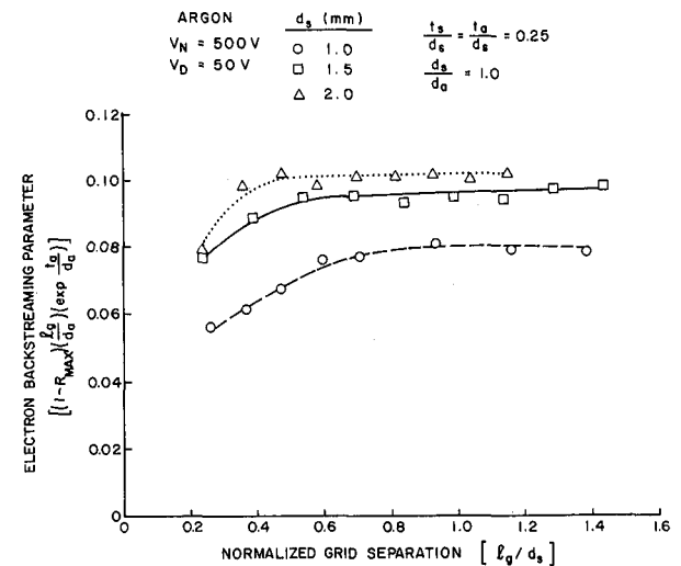
Fig. 11 Effect of Screen/Accelerator Grid Aperture Diameter on the Electron Backstreaming Parameter
