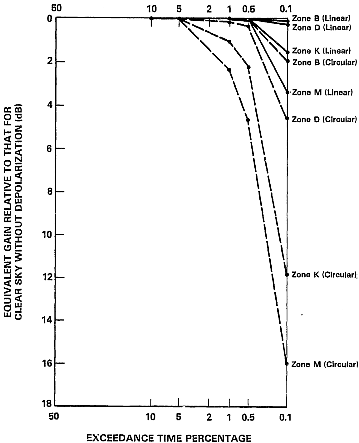
FIGURE 3.3. EQUIVALENT GAIN INCREASES DUE TO DEPOLARIZATION (SATELLITE SEPARATION = 0.5°)
