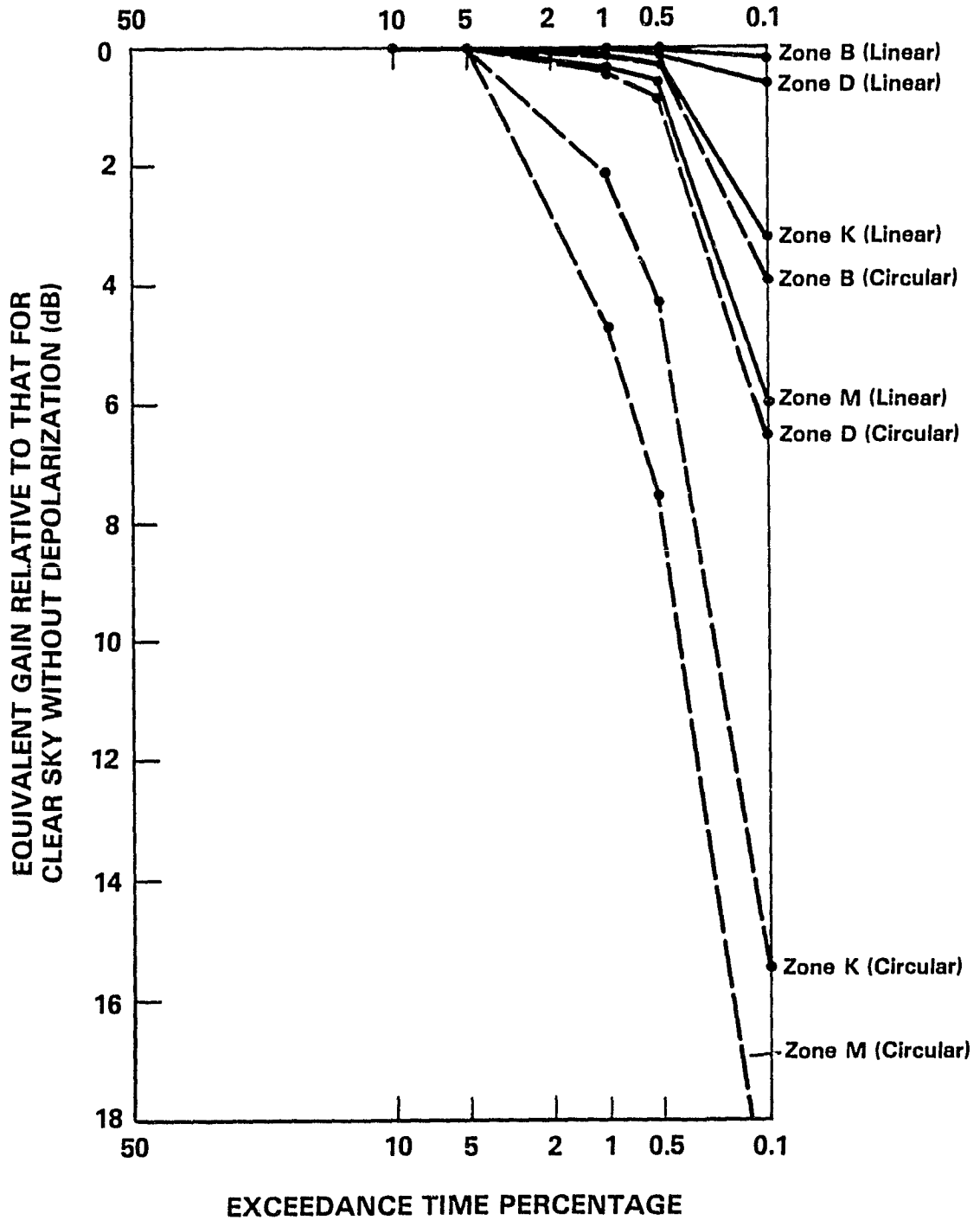
FIGURE 3.2. EQUIVALENT GAIN INCREASES DUE TO DEPOLARIZATION (SATELLITE SEPARATION = 0.3^{\circ} )
