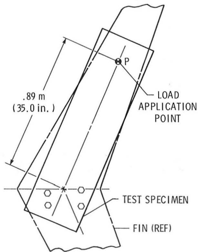
Figure 6. Fatigue Test Specimen for Vertical Fin.
