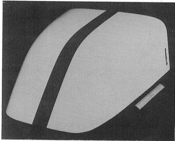
Figure 4. Bell 206L Kevlar/Epoxy Forward Fairing.
