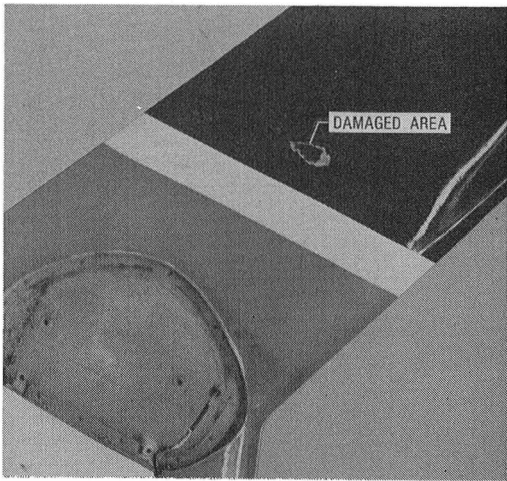
Figure 10. Damaged Bell 206L Graphite/Epoxy Composite Vertical Fin.
