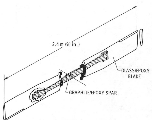
Figure 14. Sikorsky S-76 Tail Rotor Paddle
