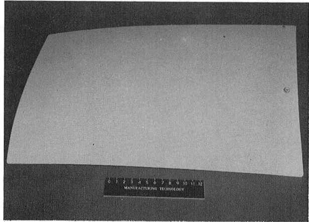
Figure 3. Bell 206L Kevlar/Epoxy Baggage Door.
