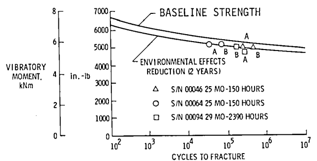
Figure 19. S-76 Tail Rotor Spar, Moment-Cycle Fatigue Curve.
