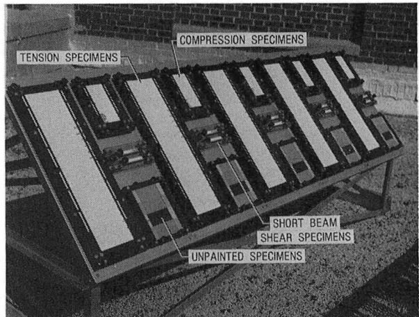
Figure 8. Environmental Exposure Rack with Specimens Installed.
