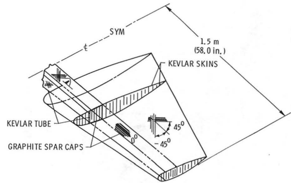
Figure 12. Composite Horizontal Stabilizer for S-76.
