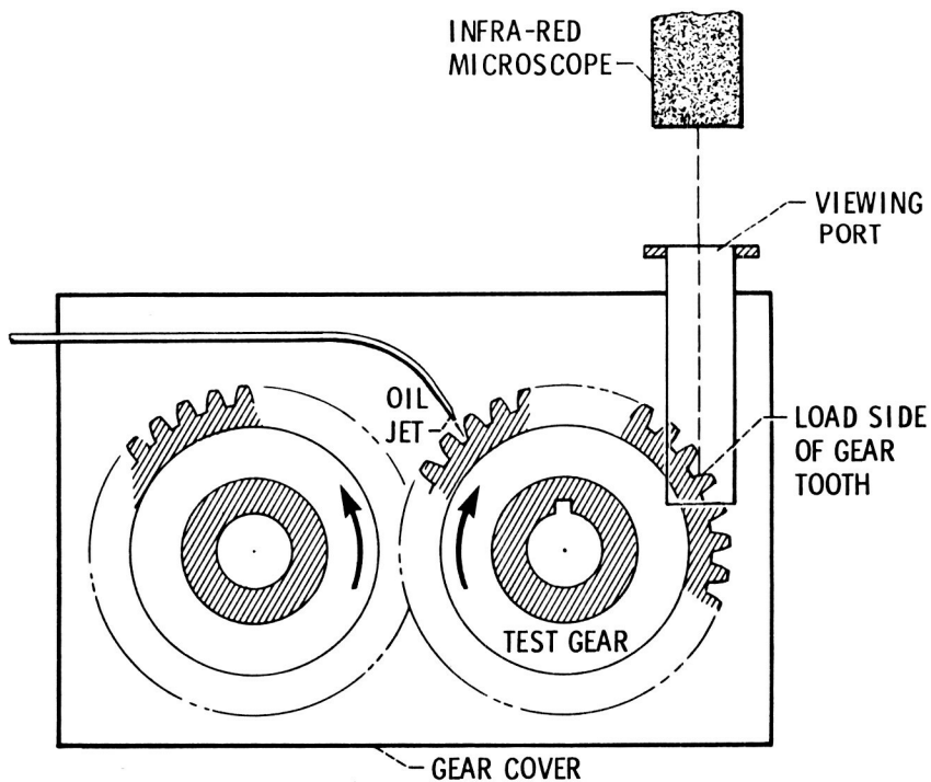
Figure 2. - Test setup for measuring dynamic gear tooth surface temperature.
