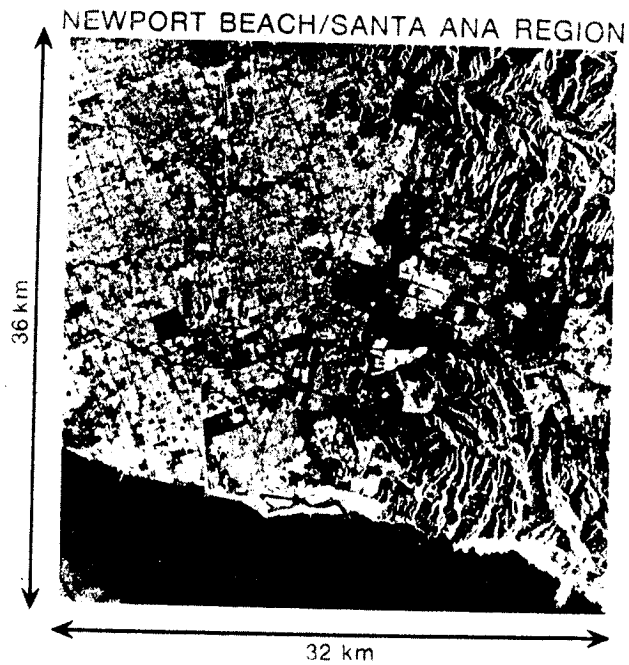
Figure 6. Seasat SAR image subsene of Newport Beach/Santa Ana, California. Note the visibility of major transportation arteries, port facilities, and urban built-up areas.
