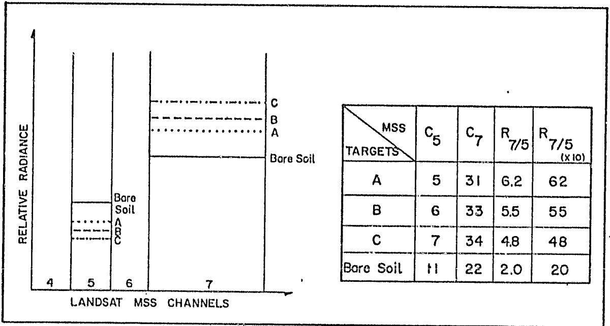
Fig. 4 - Radiance values for three areas A, B and C with varying vegetation density and one with bare soil, in channels 5 and 7.
