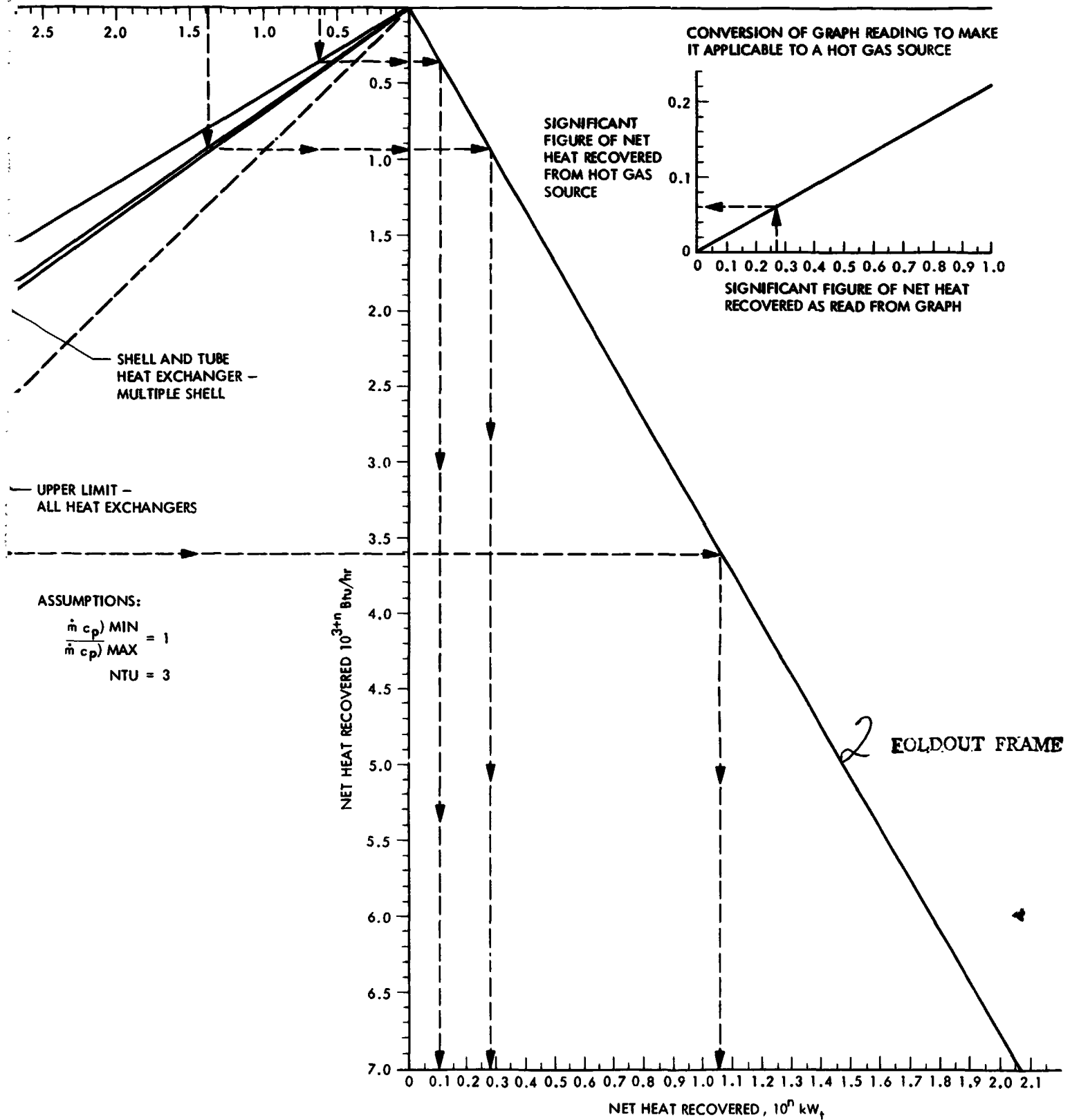
Figure 3-7. Nomogram for Determining Net Heat Recovered by a Recuperative Heat Exchanger from a Waste Heat Source
