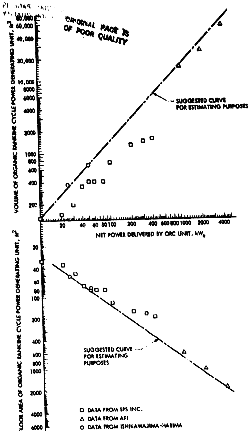
Figure 1-6. Graphical Method for Estimating Volume and Area of an Organic Rankine Bottoming Cycle Unit
