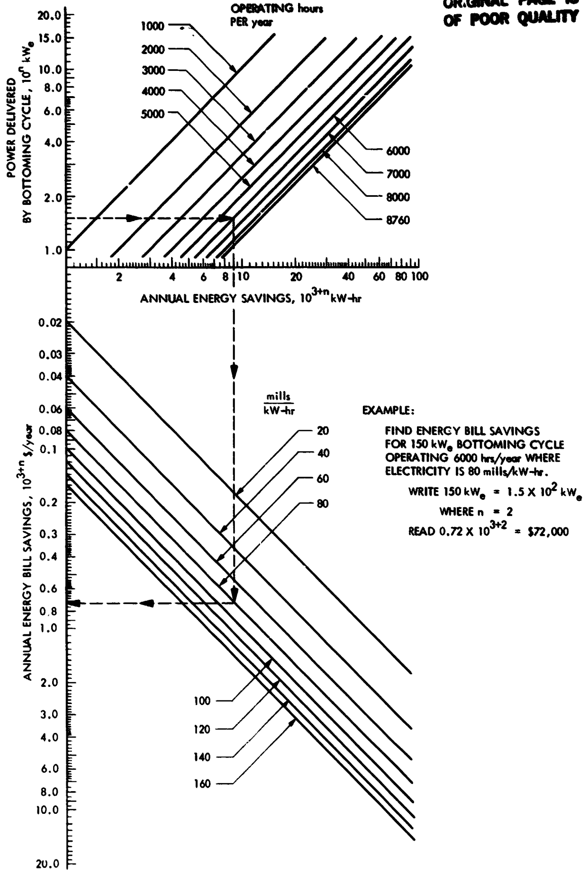
Figure 4-6. Graphical Method for Estimating Annual Energy Bill Savings
