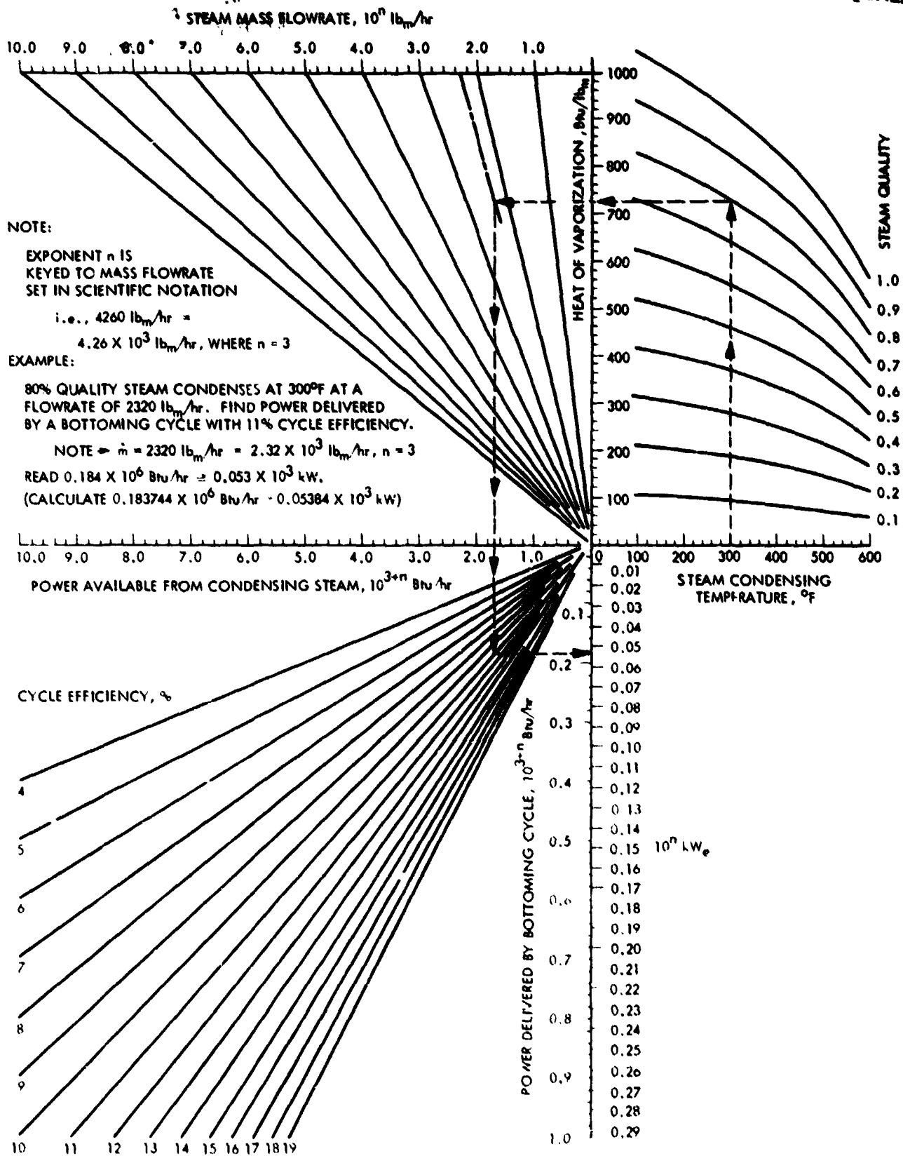
Figure 3-5. Nomogram for Determining Net Power Delivered by an Organic Rankine Cycle Fed from a Condensing Steam Waste Heat Source
