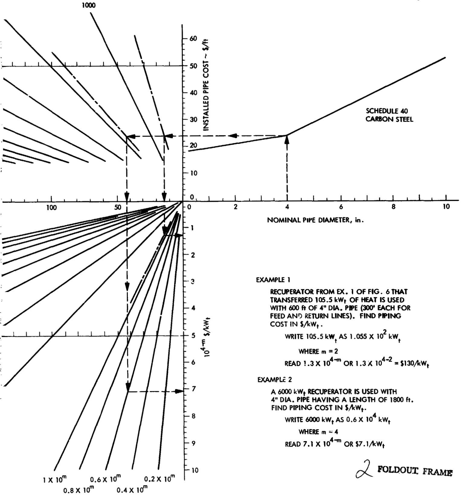
Figure 4-9. Graphical Method for Estimating Piping Costs in $/kW t
