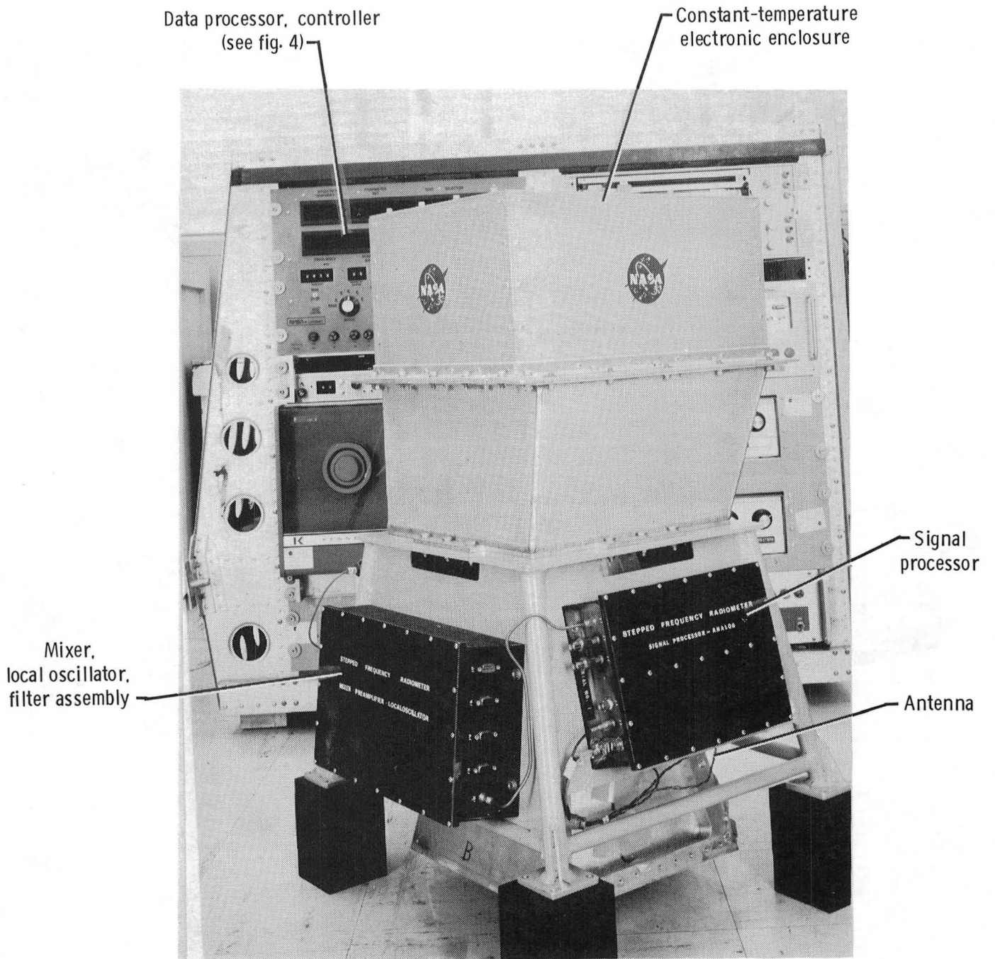
Figure 2.- Stepped frequency microwave radiometer.
