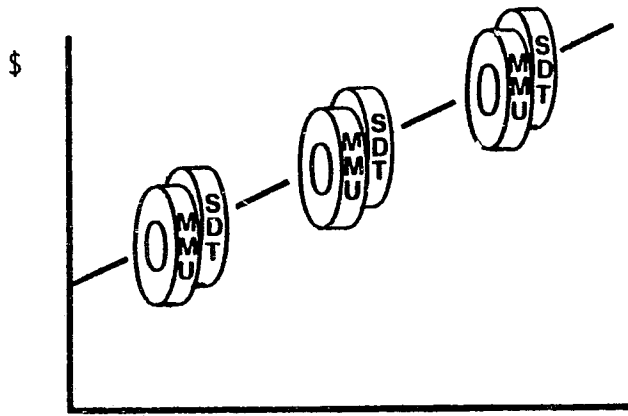
QUANTITY ALGORITHM 1
