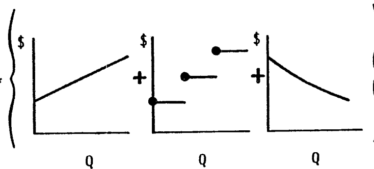
ALGORITHM 4
