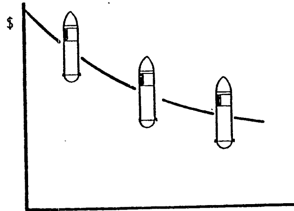
QUANTITY ALGORITHM 3
