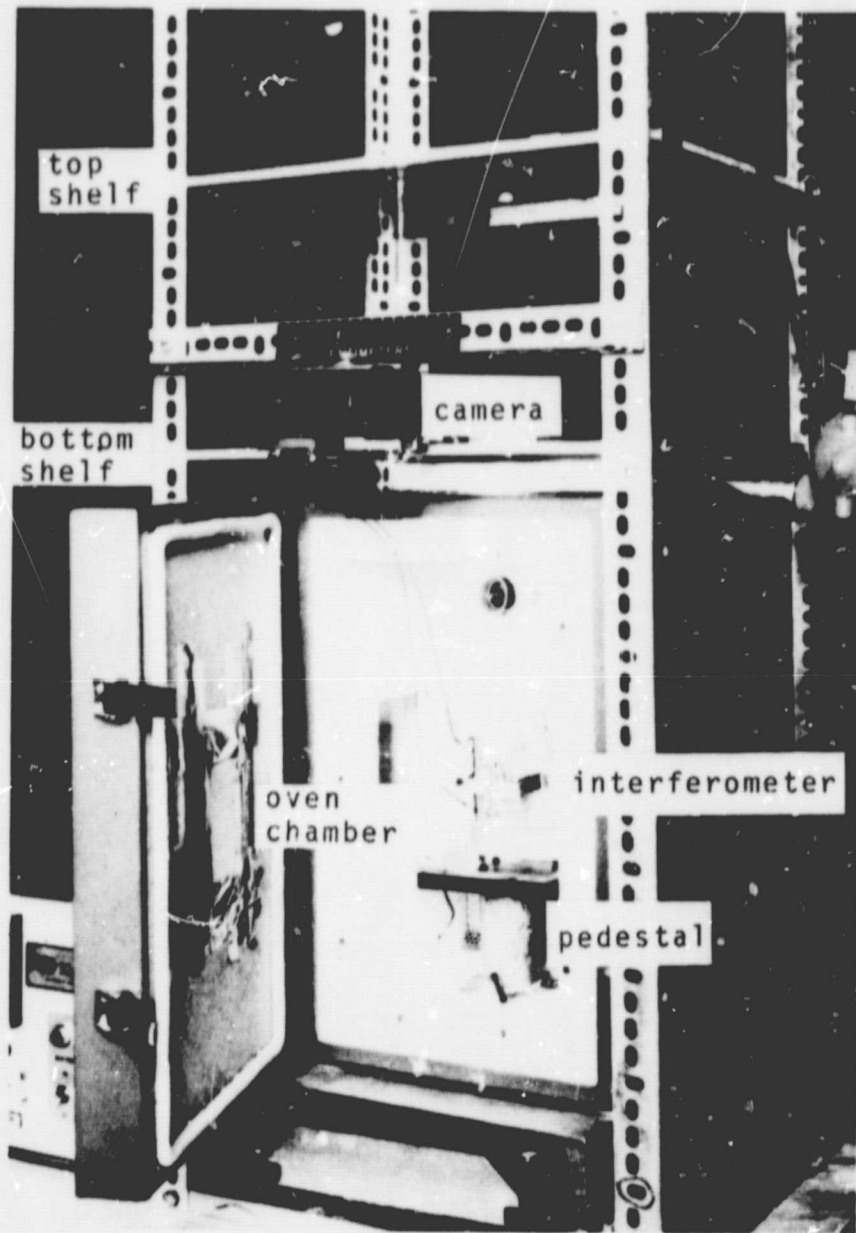
Fig. 2.5 Overall View of Experimental Apparatus
