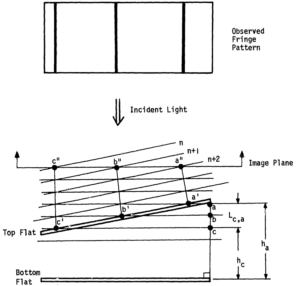
Fig. 2.3 Correspondence of Image Plane Fringes and Relative Displacement of Top Flat Ends
