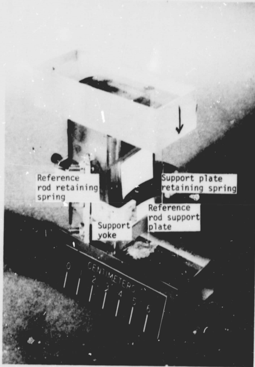
Fig. 2.7 Assembled Priest Interferometer
