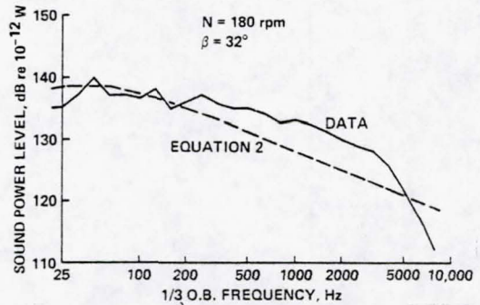
Fig. 7 Measured and predicted 1/3 O.B. spectra.
