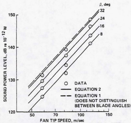
Fig. 6 Measured and predicted sound power.
