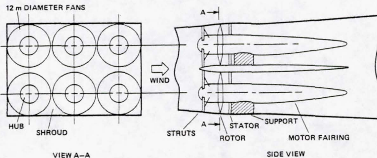
Fig. 1 Arrangement of six fan-drive units.
