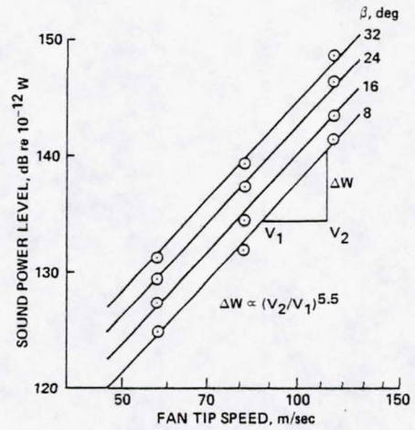
Fig. 3 Fan sound power at fixed pitch angles.
