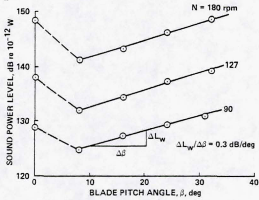
Fig. 4 Fan sound power at fixed rpm.
