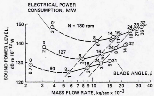
Fig. 5 Fan sound power versus mass flow.
