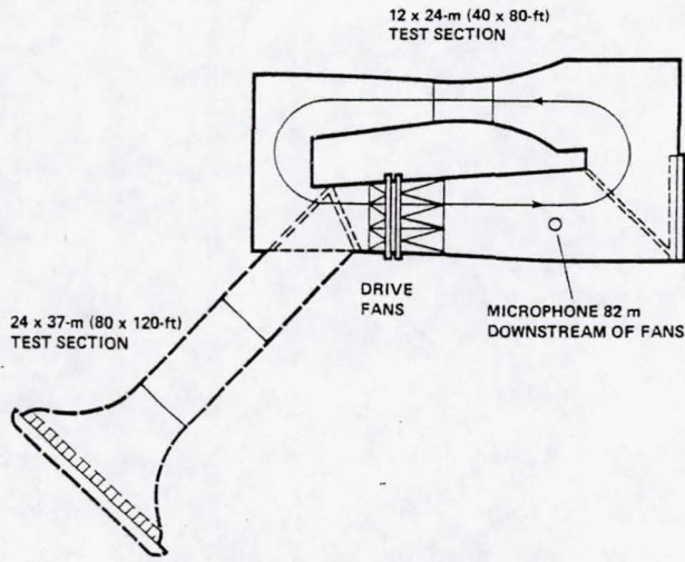
Fig. 2 Wind tunnel circuit.
