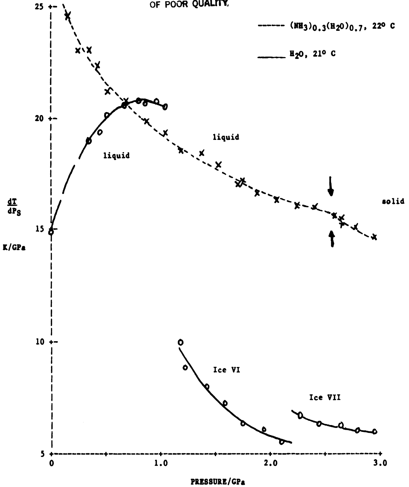
Fig. 1. Adiabats of H_2O and (NH_3)_{0.3}(H_2O)_{0.7} near 295 K
