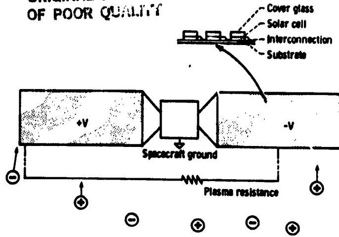
Figure 1. - Interactions between spacecraft high-voltage system and environment.
