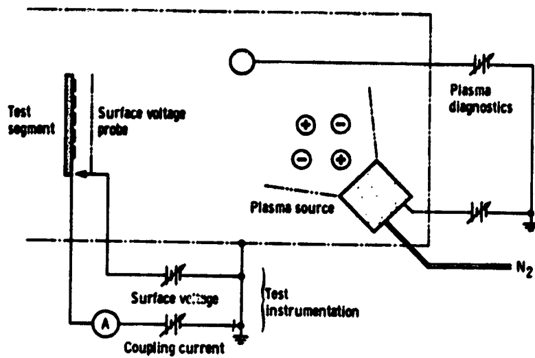
Figure 3. - Schematic diagram of test arrangement.
