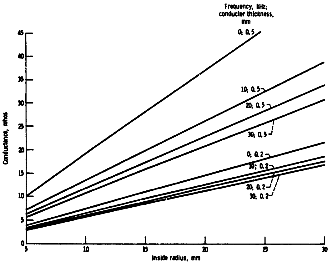
Figure 12. - Coaxial cable conductance as a function of inside radius for 50-m-long coaxial cable. Voltage, 1000 V; current, 100 A.
