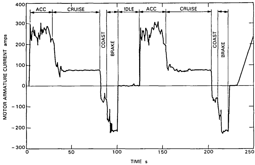
Figure 3-5a. Motor Armature History from Dynamometer Test During SAE J227a-D Driving Cycle
