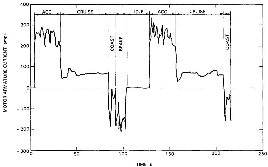
Figure 3-5b. Motor Armature History from Track Test During SAE J227a-D Driving Cycle
