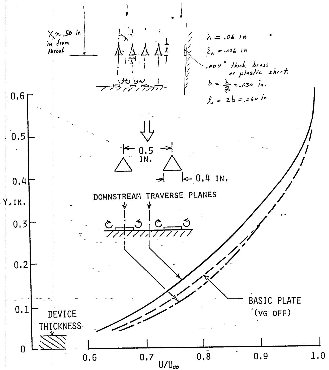
Figure 4. Boundary layer velocity profiles on plate 10 in. downstream of array of triangular elements
