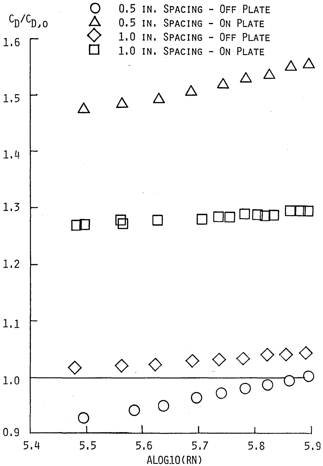
Figure 11. Drag results with vane-type VG(#2) on and off plate showing effect of spacing
