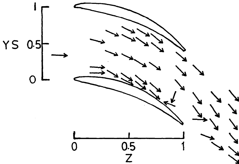
Figure 29. Limiting Streamline Angle Distribution on the IGV Endwall ( \bar{\phi} = 0.556 )
