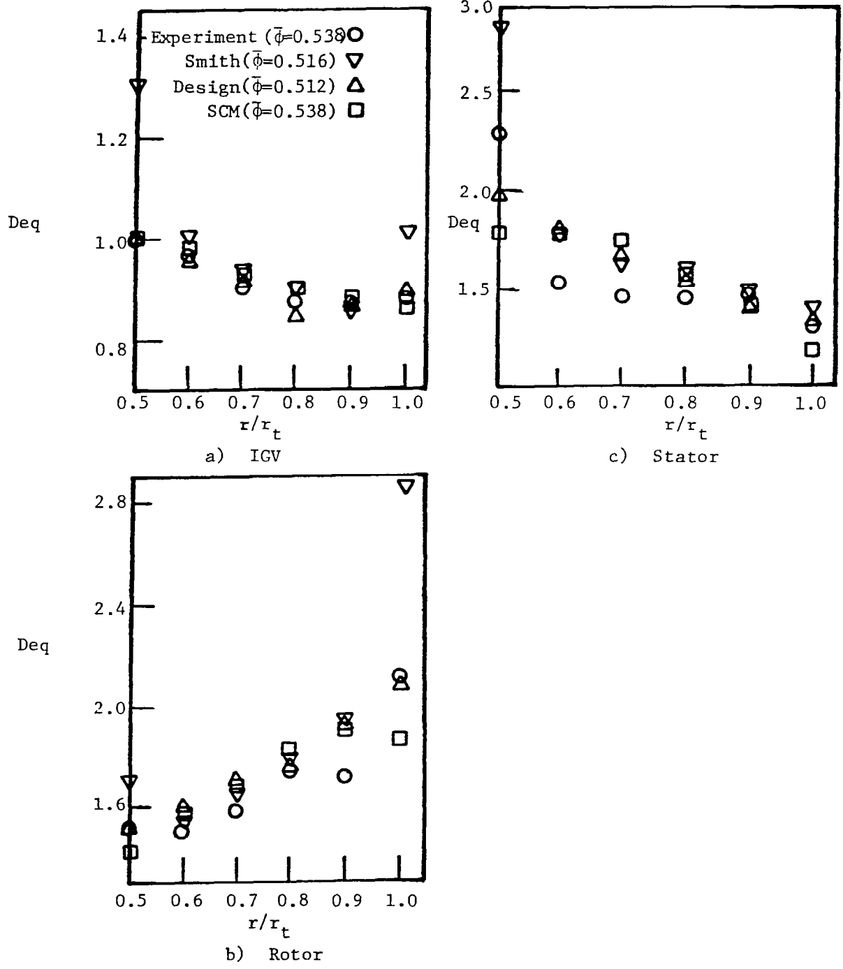
Figure 13. Blade Element Performance: Equivalent Diffusion Factor
