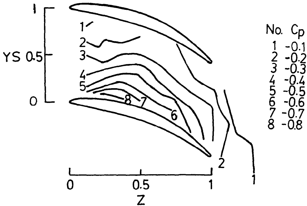
Figure 30. Static Pressure Distribution on the IGV Endwall ( \bar{\phi} = 0.556 )
