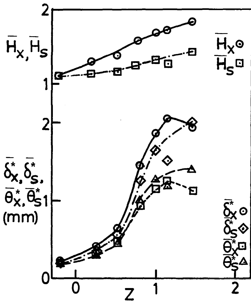
Figure 40. IGV Endwall Flow: Passage Averaged Boundary Layer Integral Parameters ( \bar{\phi} = 0.556 )
