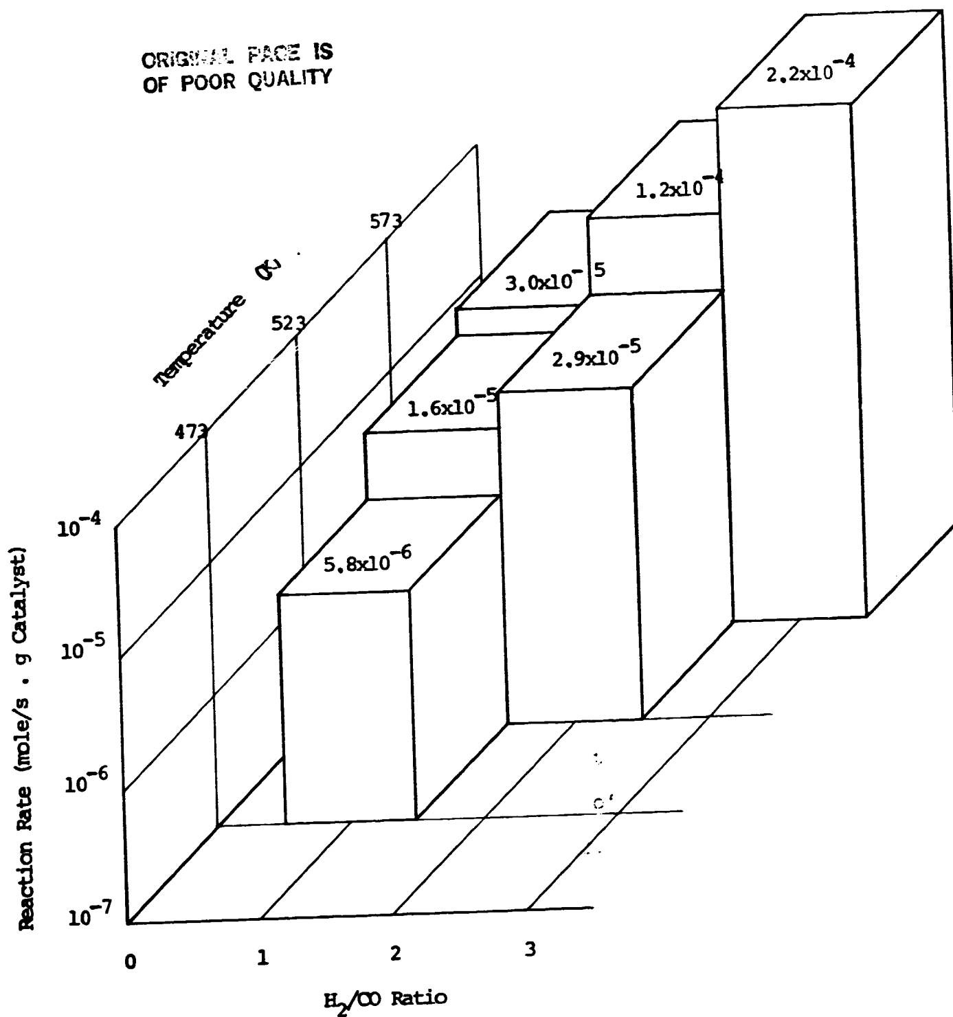
Figure 4.21 Overall Reaction Rates of 97\text{Ru}_3\text{Fe} Catalyst at Various Temperatures and \text{H}_2/\text{CO} Feed Ratios (43)
