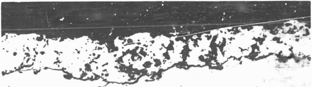
a. Loss of coating from edge and corner above failure site.
