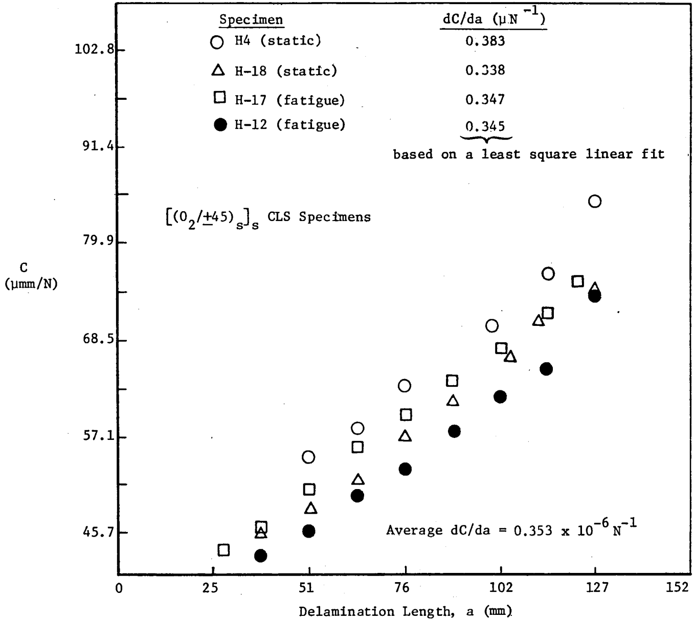
Figure 20. Compliance Variation with Delamination Size in [(0_2/\pm 45)_s]_s CLS Specimens.
