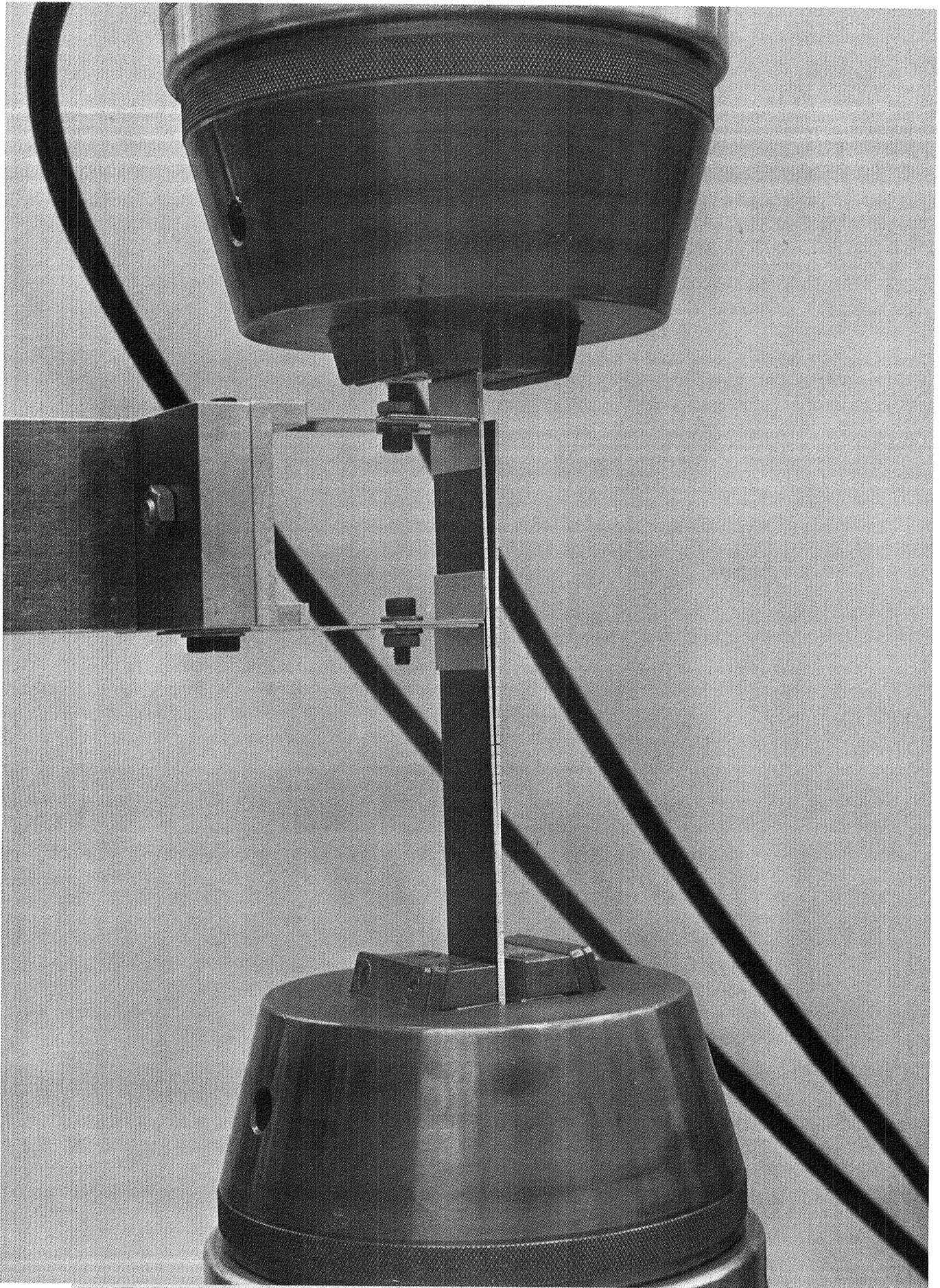
Figure 5. Cracked Lap Shear Test Setup Showing a Laterally Constrained [0_2/+45_2/0_2]_s Specimen.
