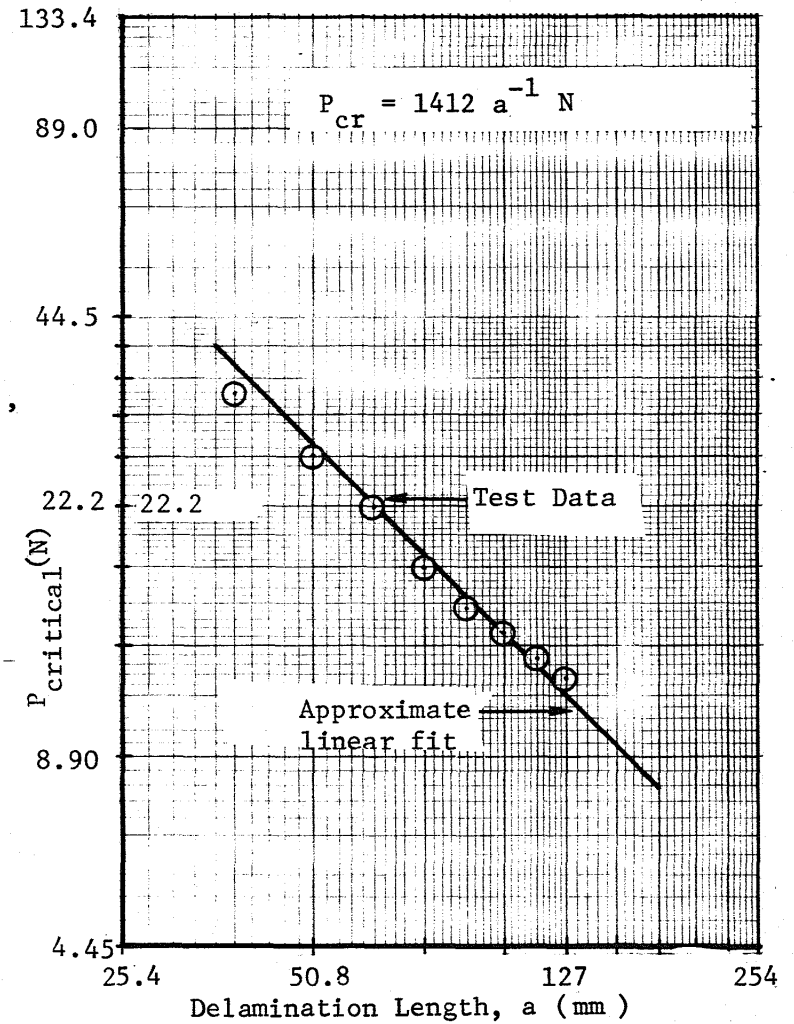
Figure 15. Static DCB Test Data From [(0_2/\pm 45)_3/0]_S T300/5208 Specimens.
