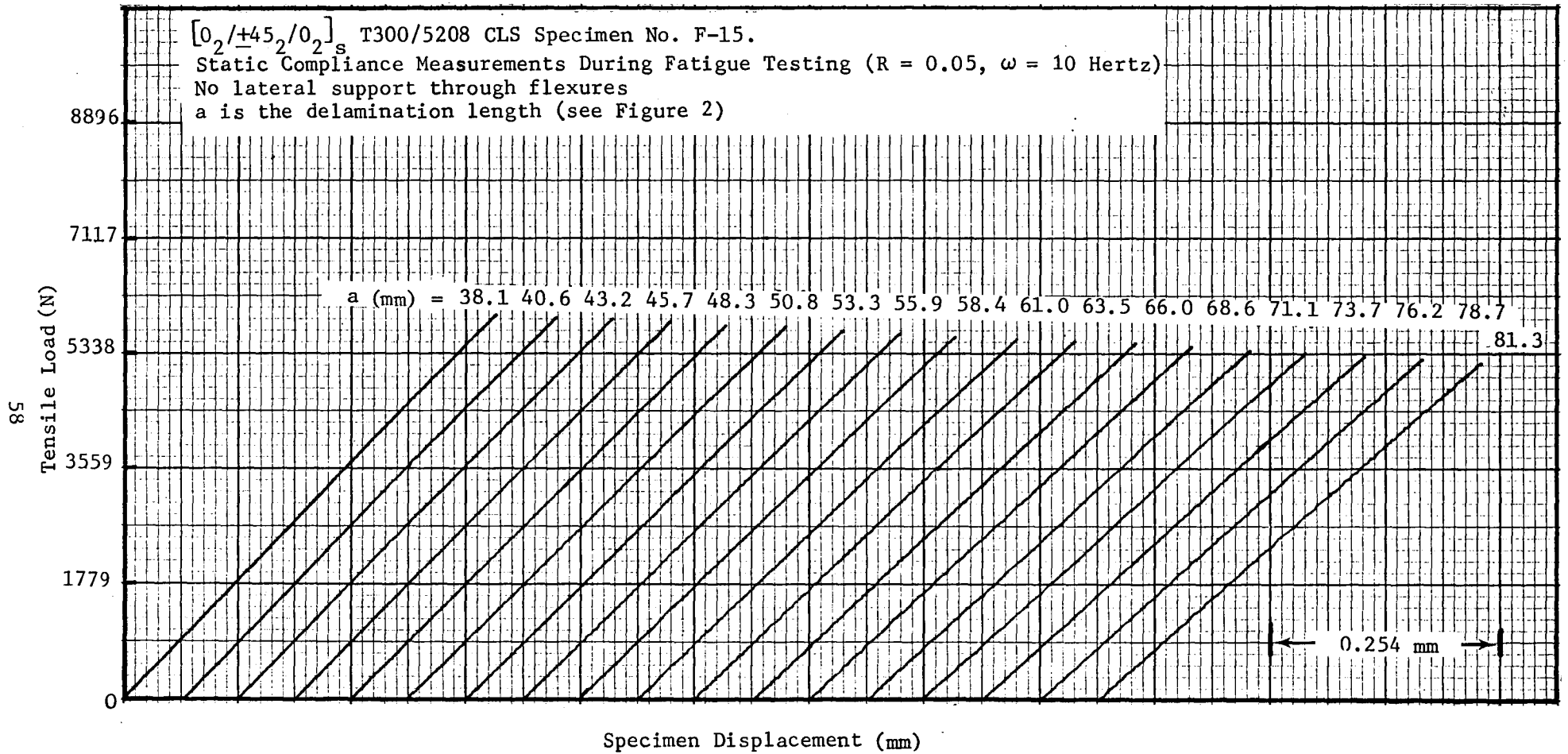
Figure 24. Typical Static Compliance Measurements During Fatigue Testing of CLS Specimens.
