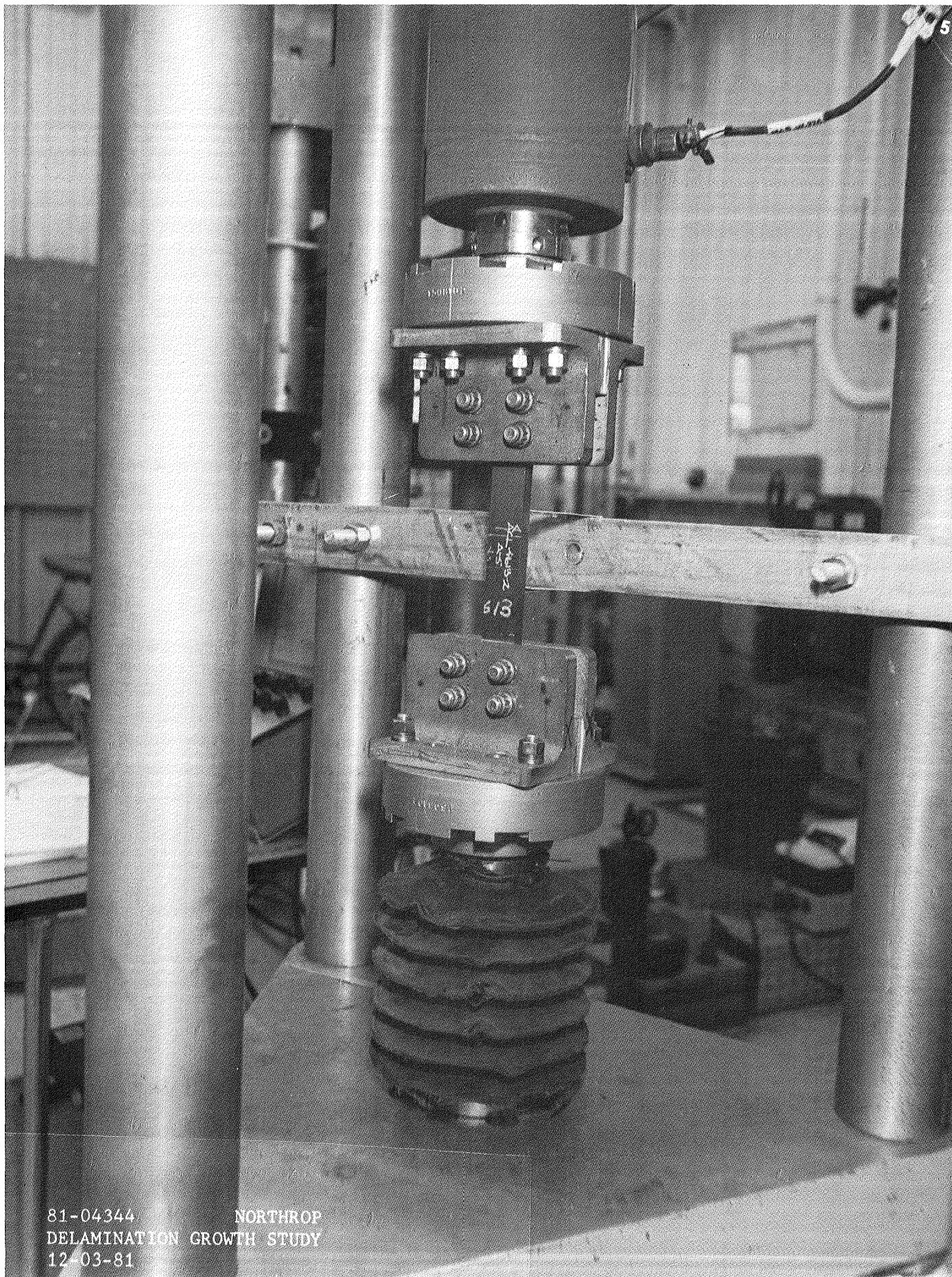
Figure 10. Compression Fatigue Test Setup For Specimens With ITW Delaminations.
