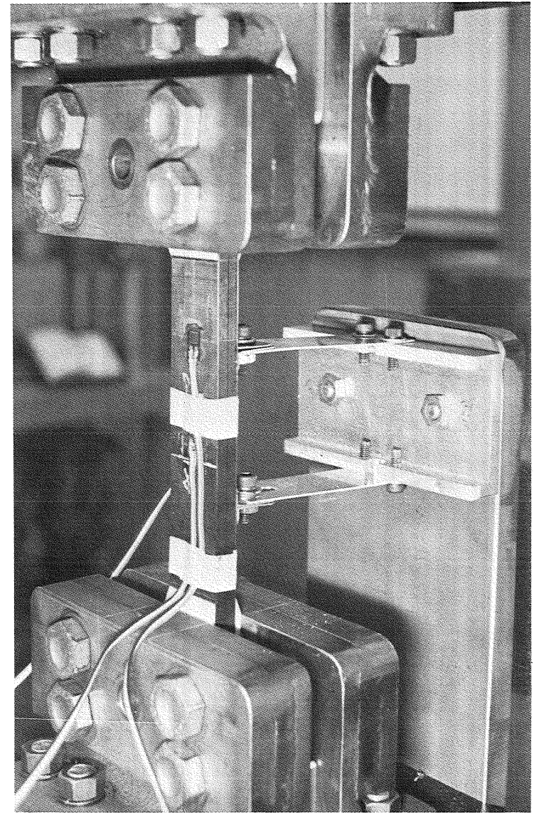
Figure 9. Static Compression Test Setup for Specimens with ITTW Delaminations. (Concluded)
