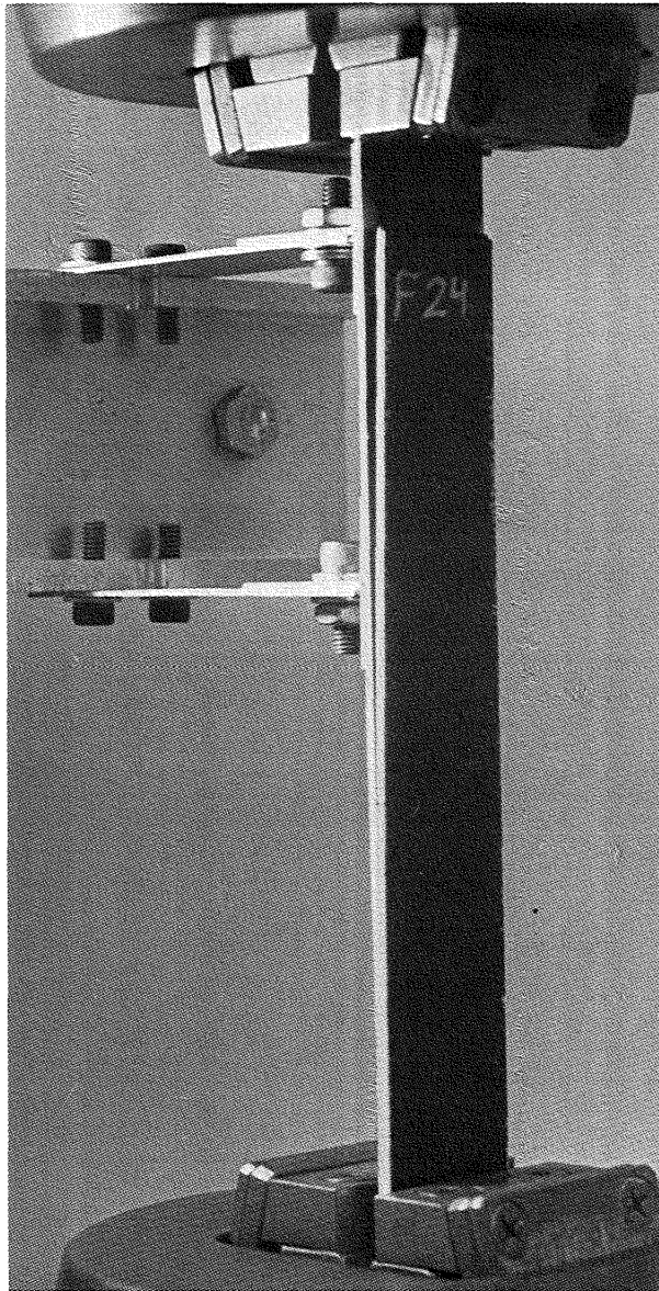
Figure 5. Cracked Lap Shear Test Setup Showing a Laterally Constrained [0_2/+45_2/0_2]_s Specimen (Concluded).
