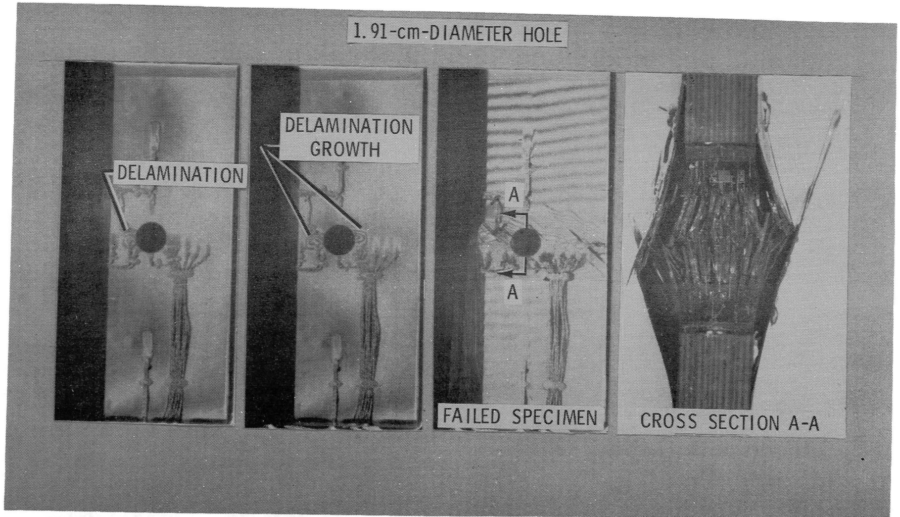
Figure 2. Local delamination failure mode in a 48-ply composite plate under in-plane compression load.
