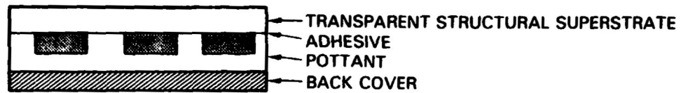
Figure 1. Flat-Plate Module Design Classifications
