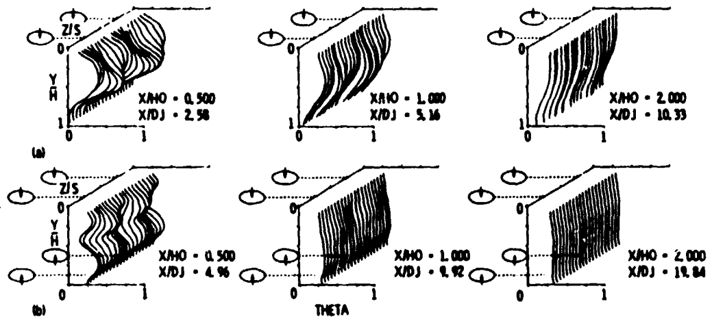
Figure 9. - Comparison between single-side and opposed jet injection ( (A)Am = .11 ).
