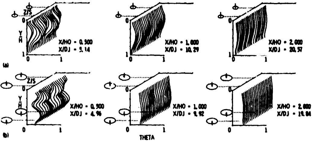
Figure 8. - Comparison between single-side and opposed jet injection ( Ho/D = 81 ).
