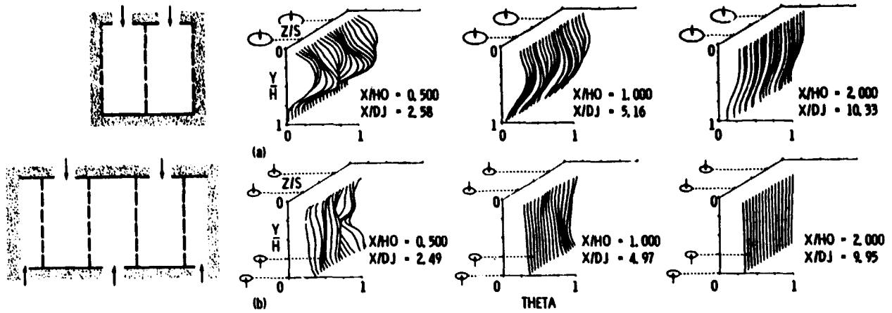
Figure 12. - Comparison between single-side and staggered jet injection ( H_0/D = 4 ; A_j/A_m = .1 ).
