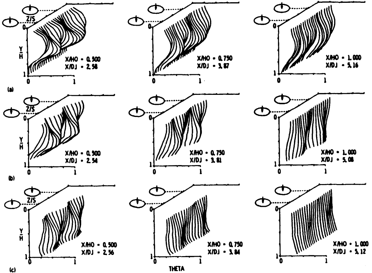
(a) Straight duct; J = 21.6 . (b) Symmetric convergence (5 cm/cm); J = 26.7 . (c) Injection wall converging (5 cm/cm); J = 26.4 .
