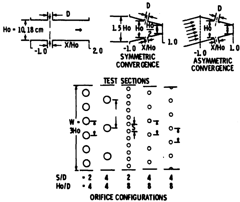
Figure 2. - Test Sections and Orifice Configurations.
