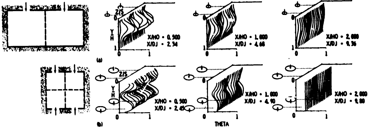
Figure 10. - Comparison between single-side and opposed injection ( H_o/D = 4 ).
