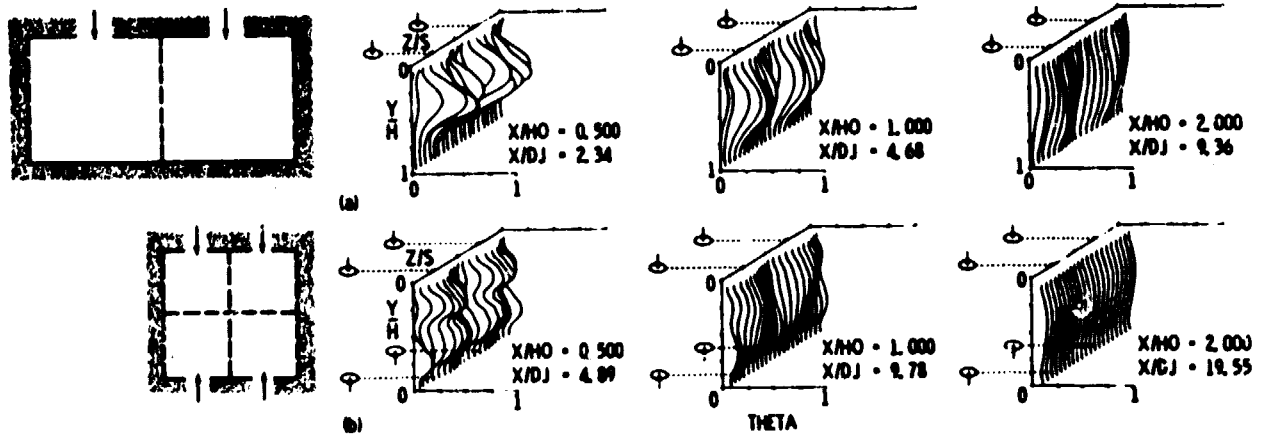
Figure 11. - Comparison between single-side and opposed jet injection ( A/JAm = .05 ).
