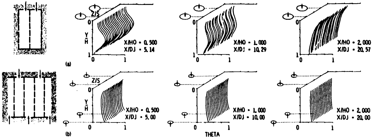
Figure 13. - Comparison between single-side and staggered jet injection ( H_0/D = 8 ; A_j/A_m = .05 ).
