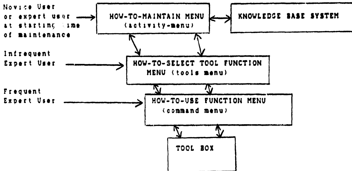
FIG. 1 Hierarchical Menu System
