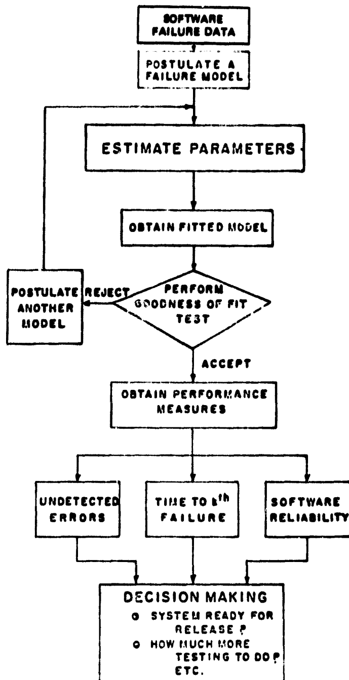
FLOWCHART FOR SOFTWARE FAILURE DATA ANALYSIS AND DECISION MAKING
