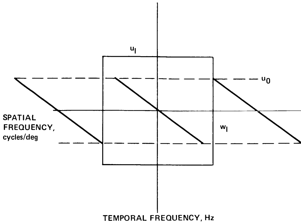
Figure 10.— Boundary condition for a moving stimulus spatially band-limited to below u_0 cycles/deg. The slope of the spectrum is r^{-1} . The first replica is just touching the window of visibility at the point w_1\mu_0 .
