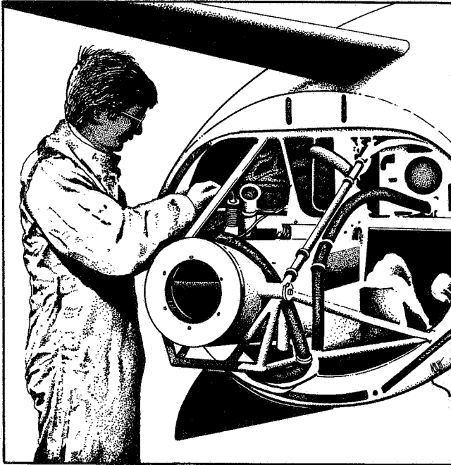
Figure 15. Airborne Airspeed Laser System (LATAS)
