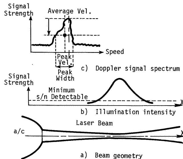
Figure 12. Principles of a CW Focused Laser Anemometer
