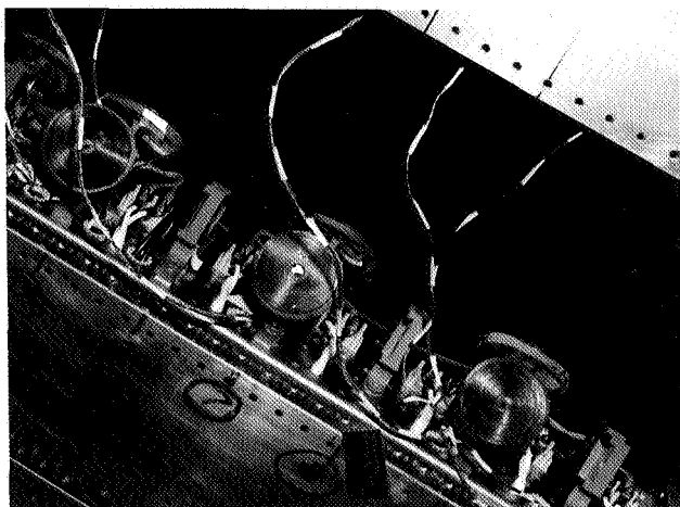
Figure 8. Closeup View of the Leading Edge of a Wing Section with the Electromagnetic Impulse System Installed
