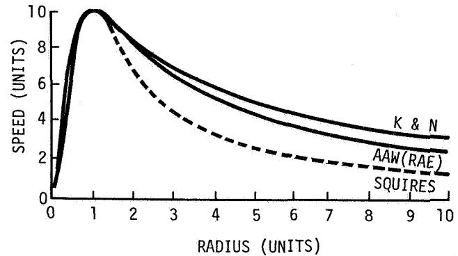
Figure 20. Comparison of Vortex Models
