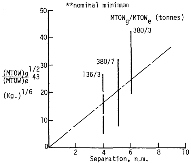
Figure 24 (b). ICAO Separation Recommendations (10 Aug. 1978)
