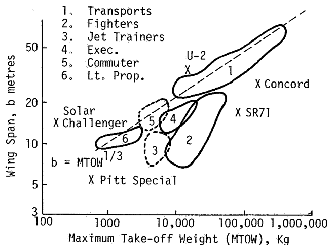
Figure 23. Aircraft Weights and Wing Span
