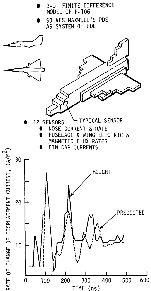
Figure 6. Comparison of Theoretical Prediction with Flight Measurements
