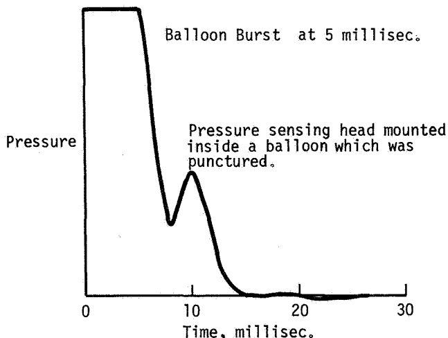
Figure 18. Response of the RAE 5-Hole Airflow Sensor To A Balloon Burst
