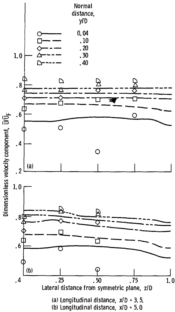
Figure 15. - Comparisons of \bar{U} component in lateral plane. Coolant injection mass flow rate, 0.22.
