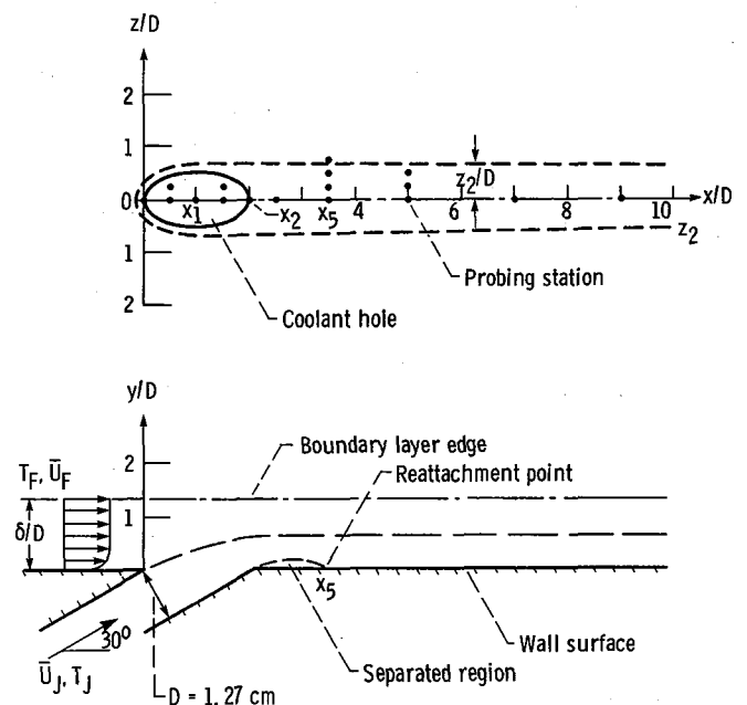
Figure 1. - Schematic of flow field.
