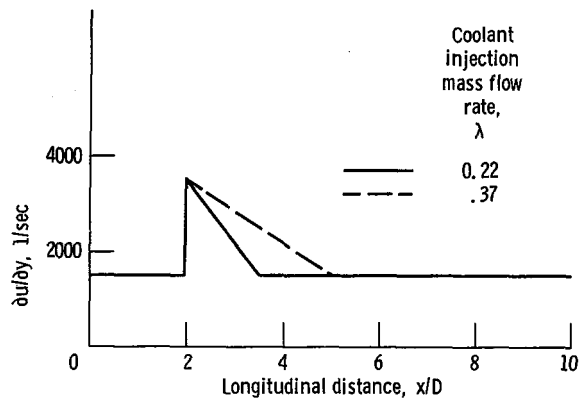
Figure 13. - Assumptions of \partial \bar{U} / \partial y in z=0 plane for numerical computation.
