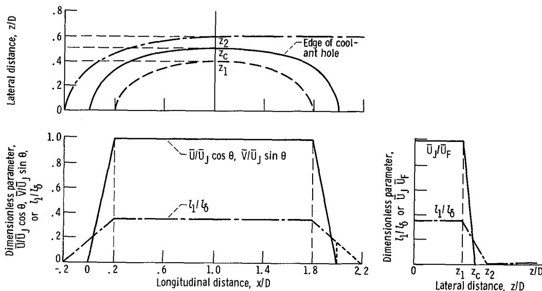
Figure 12. - Velocity and turbulent mixing length assumptions over coolant exit ( y=0 ).
