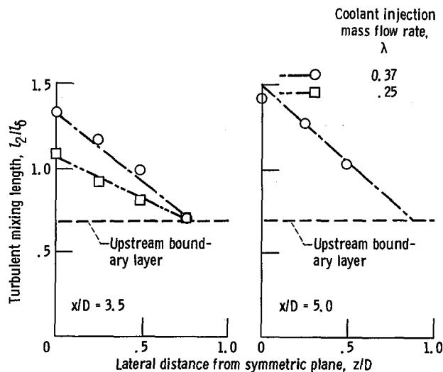
Figure 9. - Lateral variations of mixing length at pivot point 2.
