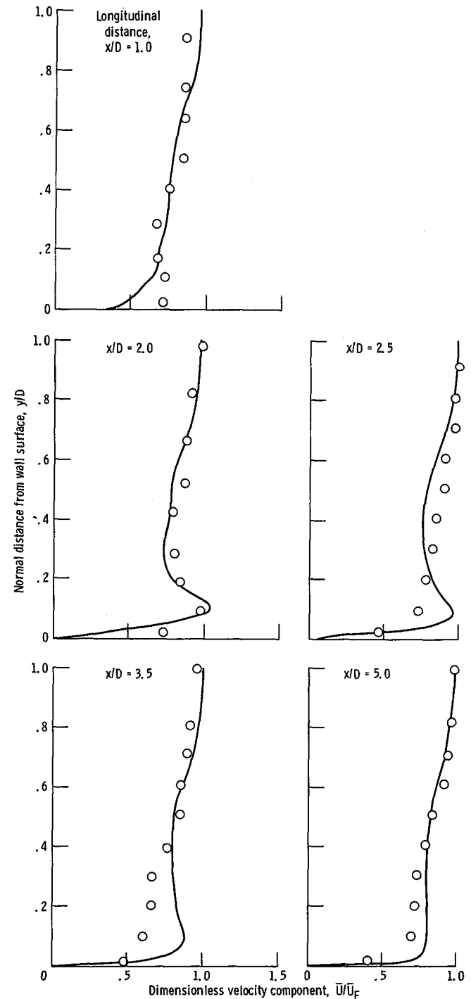
Figure 16. - Comparisons of \bar{U} components in the z plane. Coolant injection mass flow rate, 0.37.
