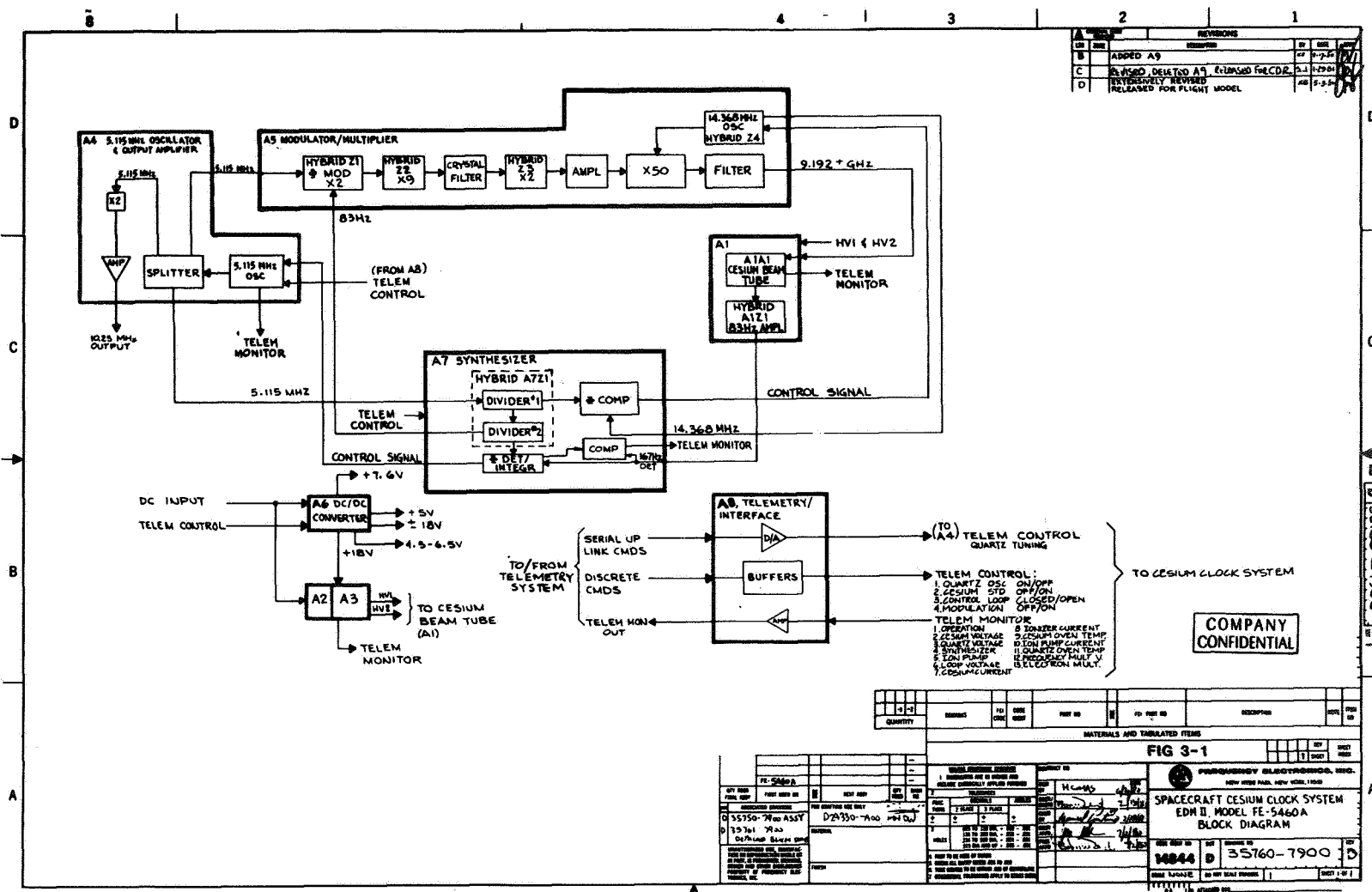
Figure 3 Spacecraft Cesium Clock System EDM II, Model FF-5460, Block Diagram
