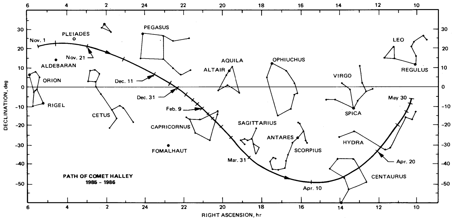
Path of Comet Halley on the Celestial Sphere During November 1985-May 1986
