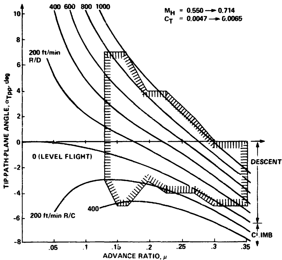
Fig. 6. OLS model testing envelope.
