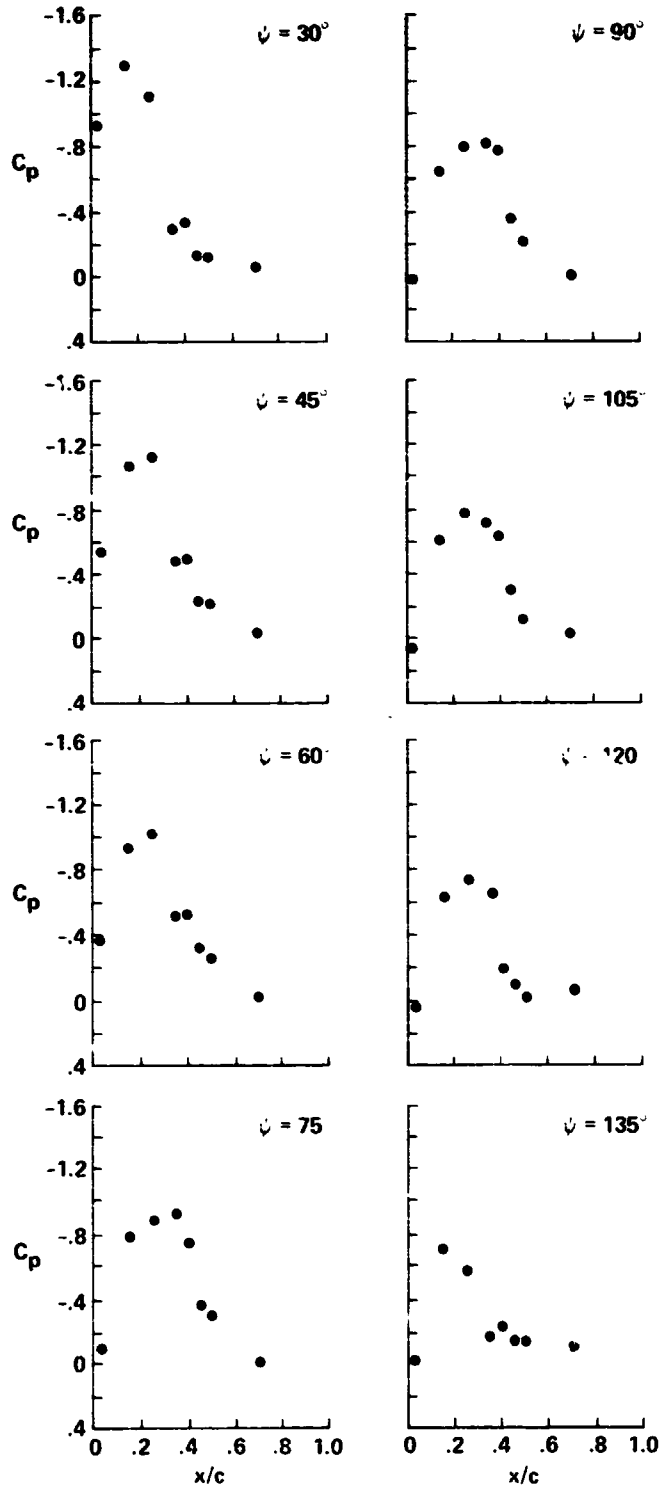
Fig. 15. Model OLS rotor upper-surface chordwise pressure coefficient versus azimuth for M_{AT} = 0.896 , 95.5% R.
