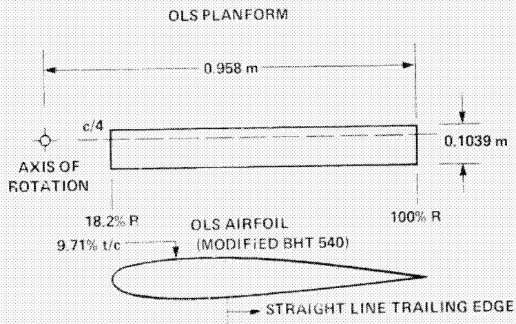
(a) OLS blade geometry.
