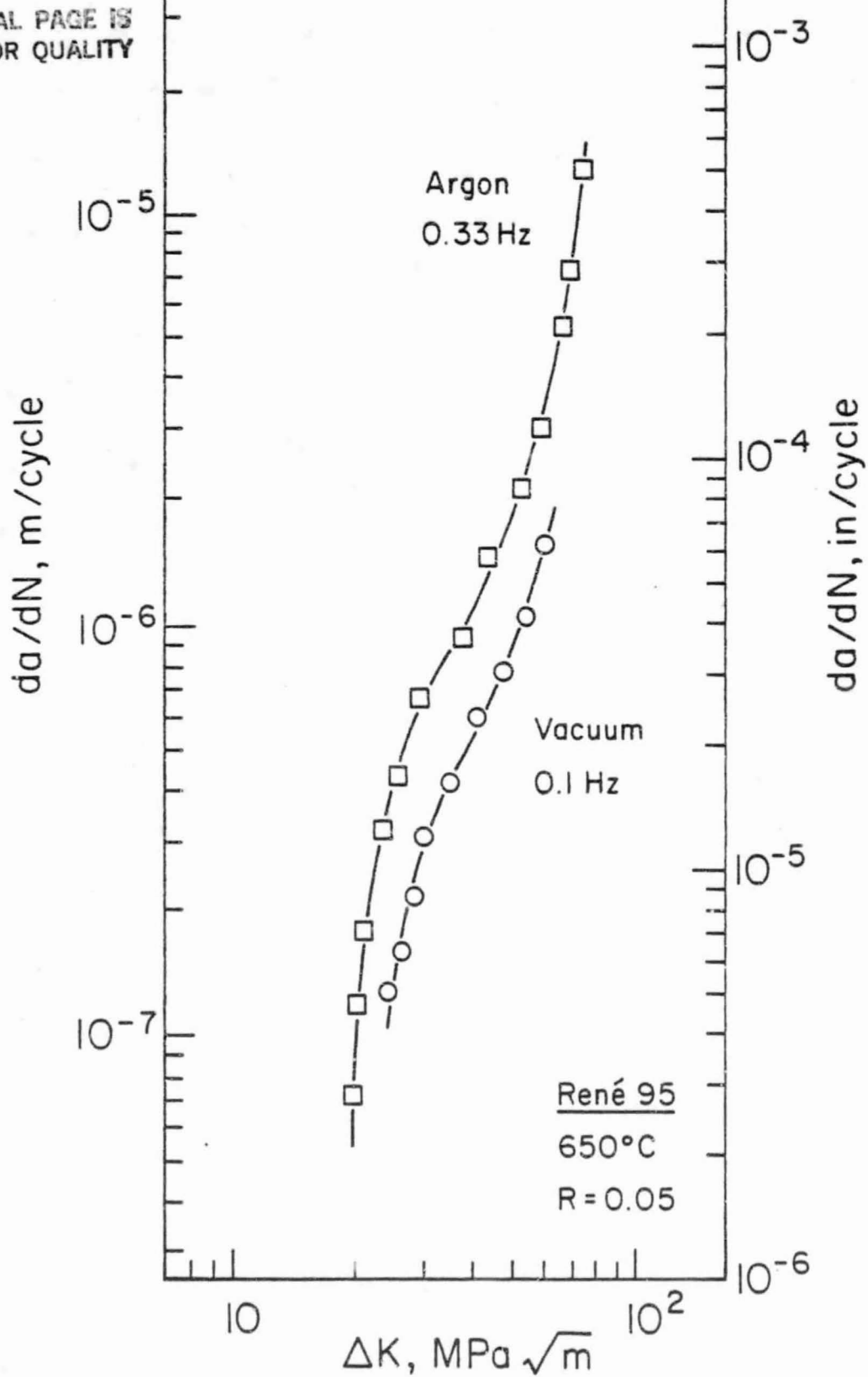
Fig. 9 Effects of environment on FCG of René 95
