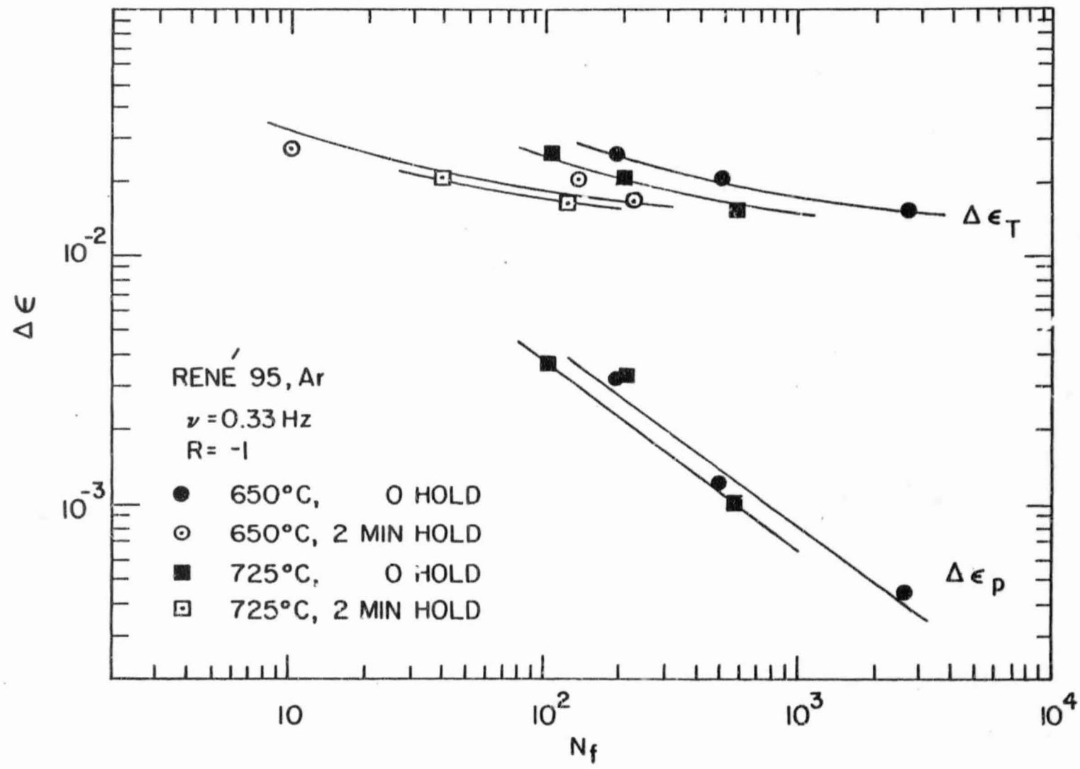
Fig. 20 LCF test results for HIP René 95
