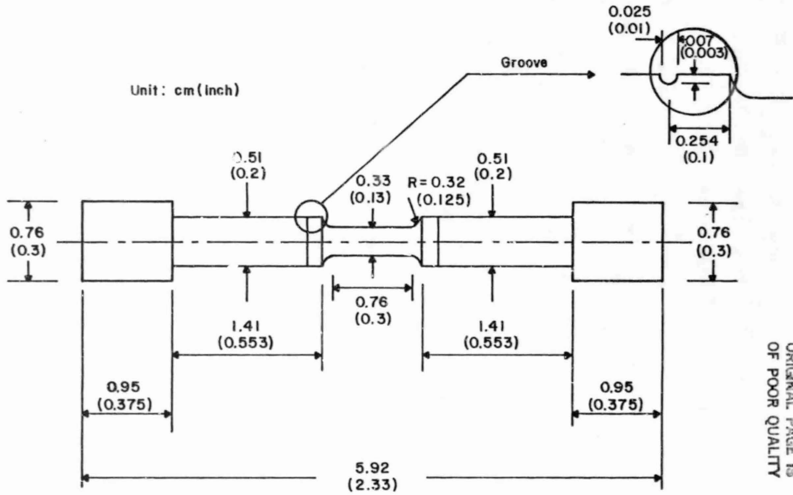
Fig. 3 Low cycle fatigue specimen design
