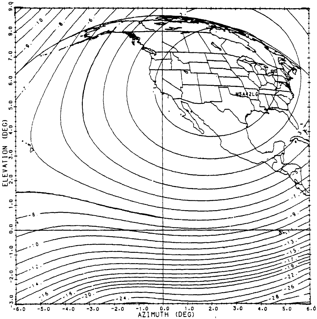
Figure 4.2-3. Satellite Antenna Beam Coverage of U.S. from 120°W
