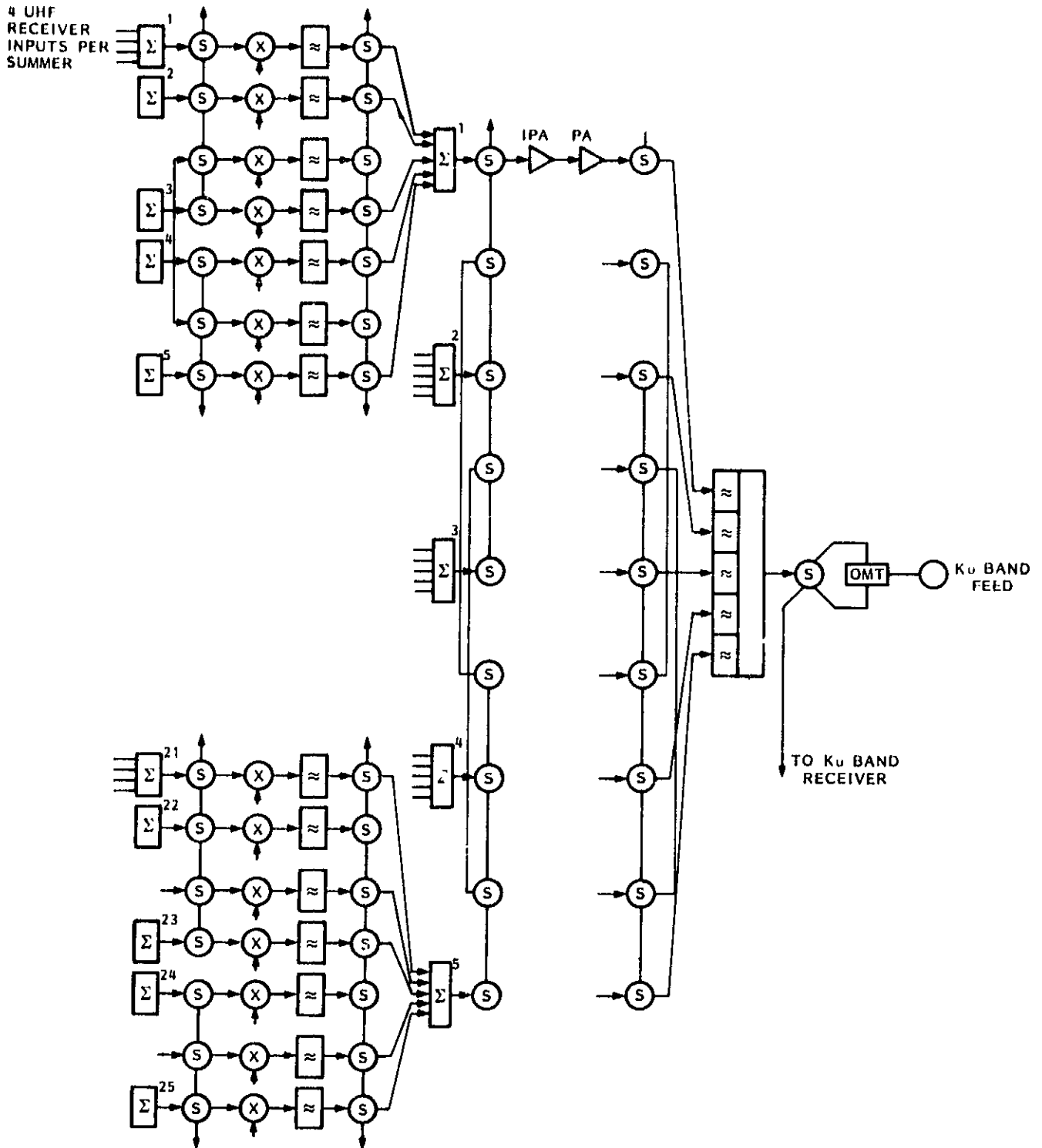
Figure 4.2-36. Concept D' Ku Band Transmitter Assembly
