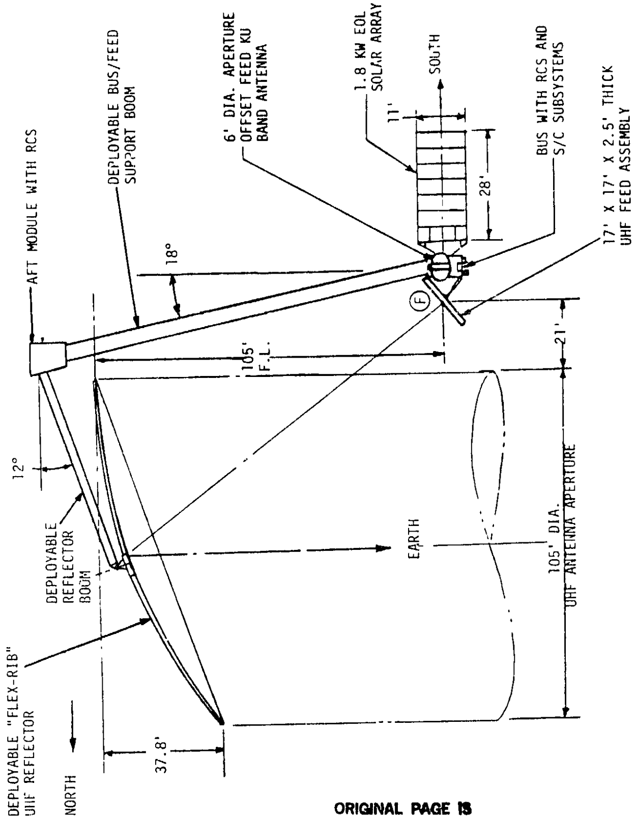
Figure 4.9-1. Orbital Geometry
