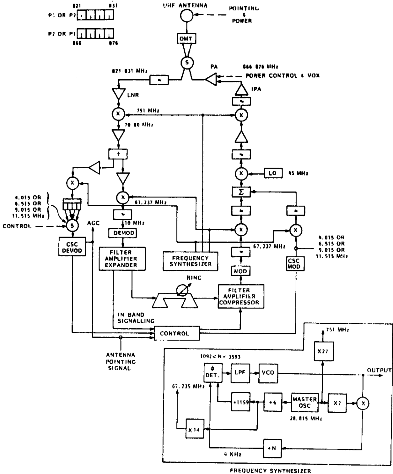
Figure 4.6-3. Radio Telephone or Dispatch (Stand-Alone) Transceiver
