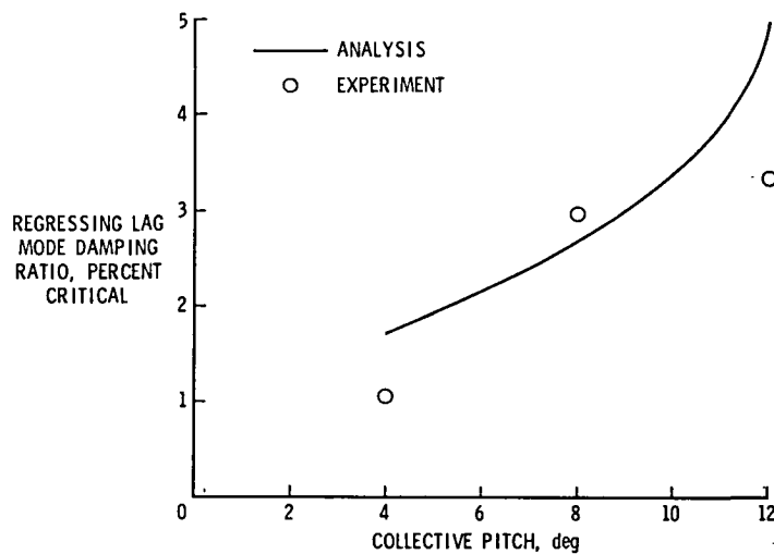
(c) Advance ratio = 0.30
