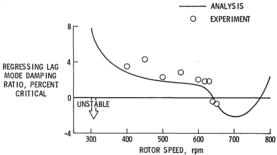
(b) Regressing lag mode damping ratio
