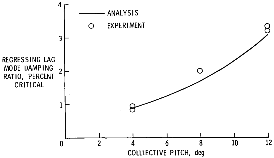
(a) Advance ratio = 0.20
