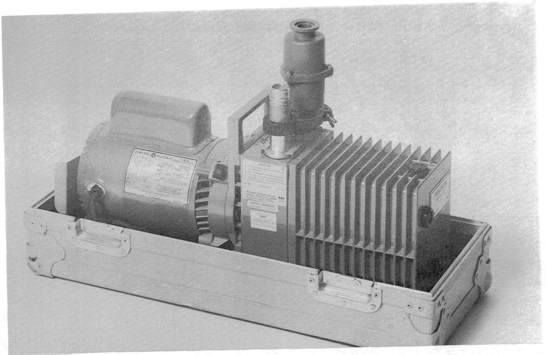
Figure 8—SEADS GTMS Portable Mechanical Pump
