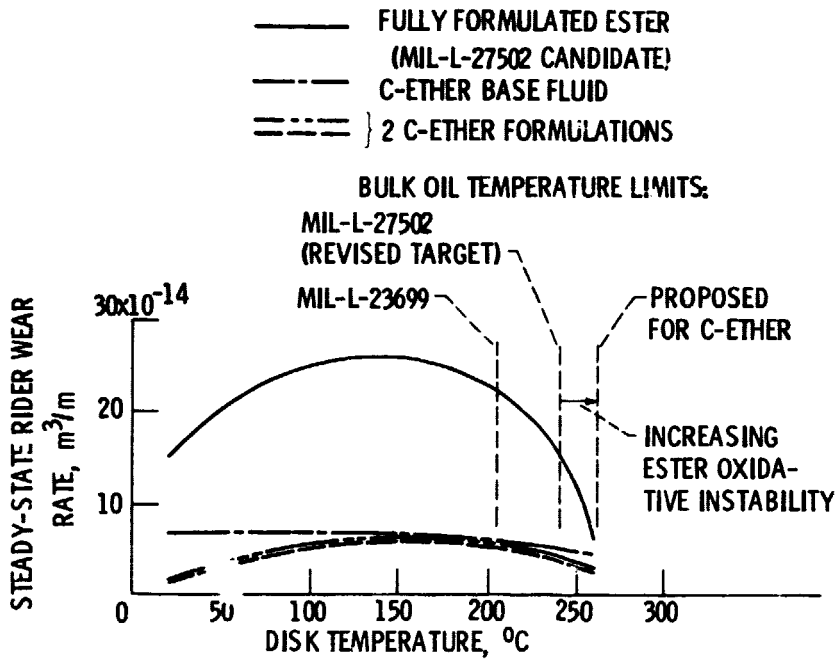
Figure 4. - Steady-state wear as a function of disk temperatures from 20° to 260° C for a formulated ester and C-ether fluids.
