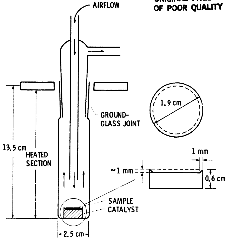
Figure 5. - Micro-oxidation apparatus.
