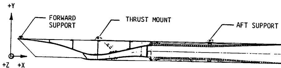
Figure 18. Engine Mount Location
