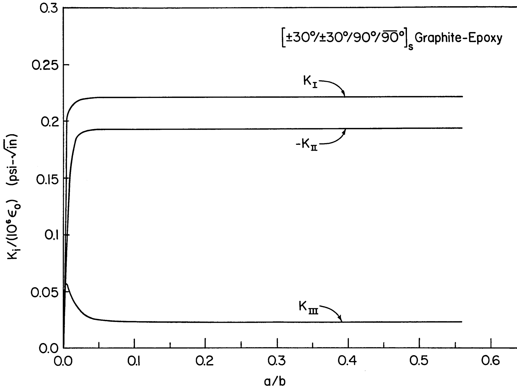
Fig. 12 Change of Stress Intensity Solutions K_I with Delamination Length a/b in [(\pm 30^\circ) / (\pm 30^\circ) / 90^\circ / 90^\circ]_s Graphite-Epoxy Subjected to Uniform Axial Strain \epsilon_z = \epsilon_0 ( h_1 = h_2 = \dots = h_{11} = 0.0054 in., b = 0.75 in.).
