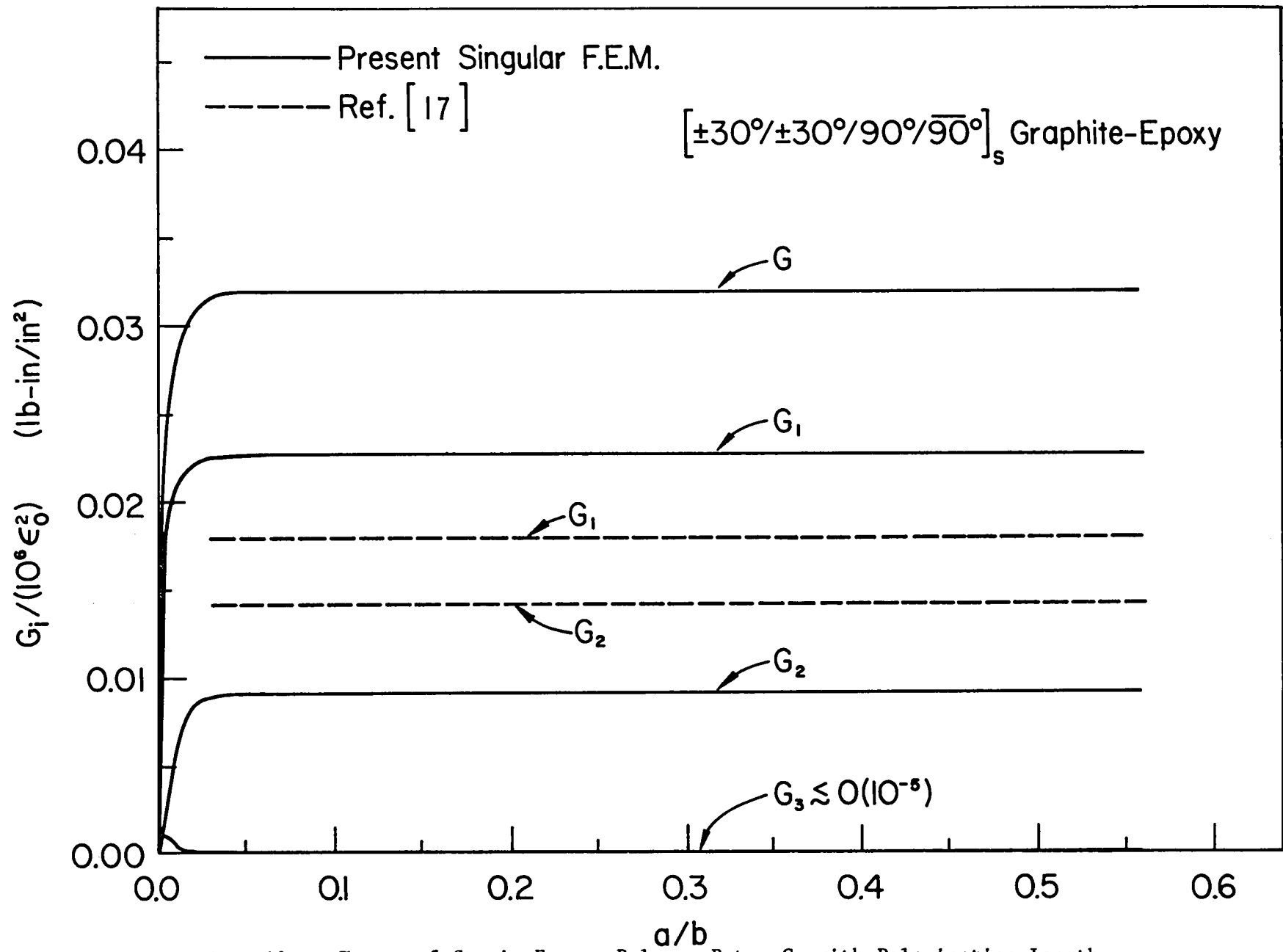
Fig. 13 Change of Strain Energy Release Rates G_i with Delamination Length a/b in [(\pm 30^\circ) / (\pm 30^\circ) / 90^\circ / 90^\circ]_s Graphite-Epoxy Subjected to Uniform Axial Strain \epsilon_z = \epsilon_0 ( h_1 = h_2 = \dots = h_{11} = 0.0054 in., b = 0.75 in.).
