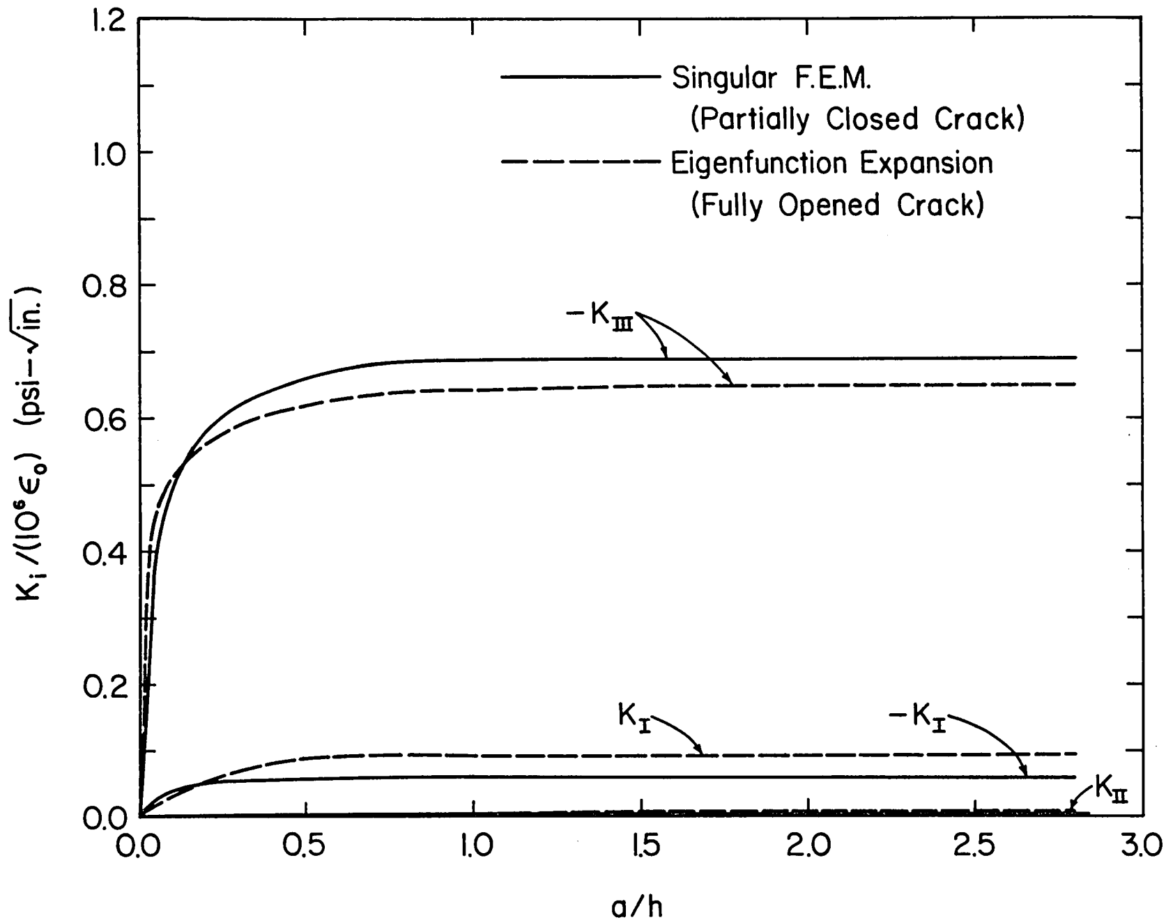
Fig. 4 Comparison of Stress Intensity Solutions Obtained by Two Different Models for Delamination in [45^\circ/-45^\circ/-45^\circ/45^\circ] Graphite-Epoxy Subjected to Uniform Axial Strain \epsilon_z = \epsilon_0 ( h_1 = h_2 = h = 0.25 in., b/h = 8 in., a = 0.25 in.).
