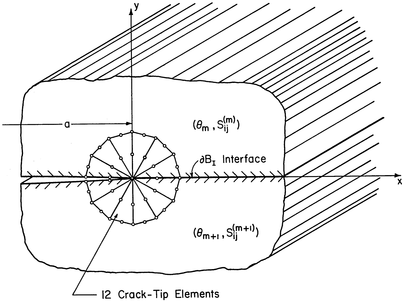
Fig. 2 Arrangement of Special Crack-Tip Elements for the Composite Delamination Problem.
