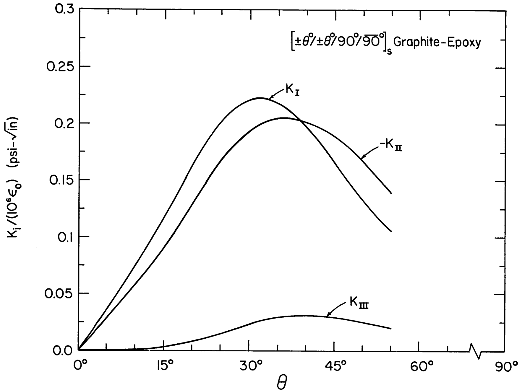
Fig. 6 Variation of Stress Intensity Factors K_i with Fiber Orientation \theta for Delamination in [(\pm\theta)/(\pm\theta)/90^\circ/90^\circ]_s Graphite-Epoxy under Uniform Axial Strain \epsilon_z = \epsilon_0 ( h_1 = h_2 = \dots = h_{11} = 0.0054 in., b = 0.75 in., \alpha = 0.5b ).
