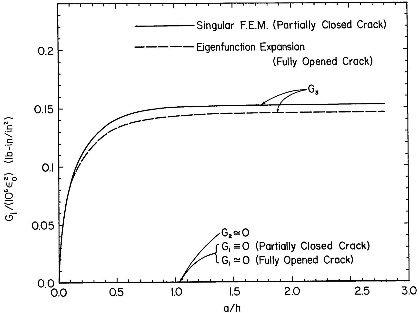
Fig. 5 Comparison of Energy Release Rates Determined by Two Different Models for Delamination in [45^\circ/-45^\circ/-45^\circ/45^\circ] Graphite-Epoxy Subjected to Uniform Axial Strain \epsilon_z = \epsilon_0 ( h_1 = h_2 = h = 0.25 in., b/h = 8 , a = 0.25 in.).
