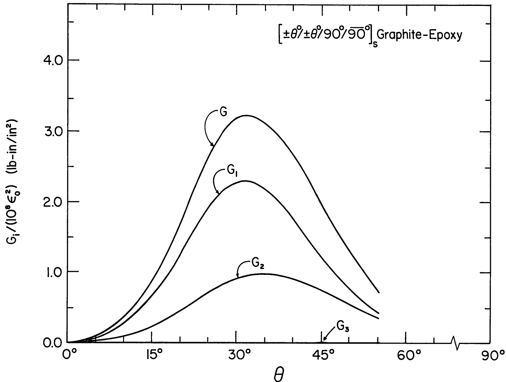
Fig. 7 Variation of Strain Energy Release Rates G_i with Fiber Orientations \theta for Delamination in [(\pm\theta)/(\pm\theta)/90^\circ/90^\circ]_s Graphite-Epoxy under Uniform Axial Strain \epsilon_z = \epsilon_0 ( h_1 = h_2 = \dots = h_{11} = 0.0054 in., b = 0.75 in., a = 0.5b ).
