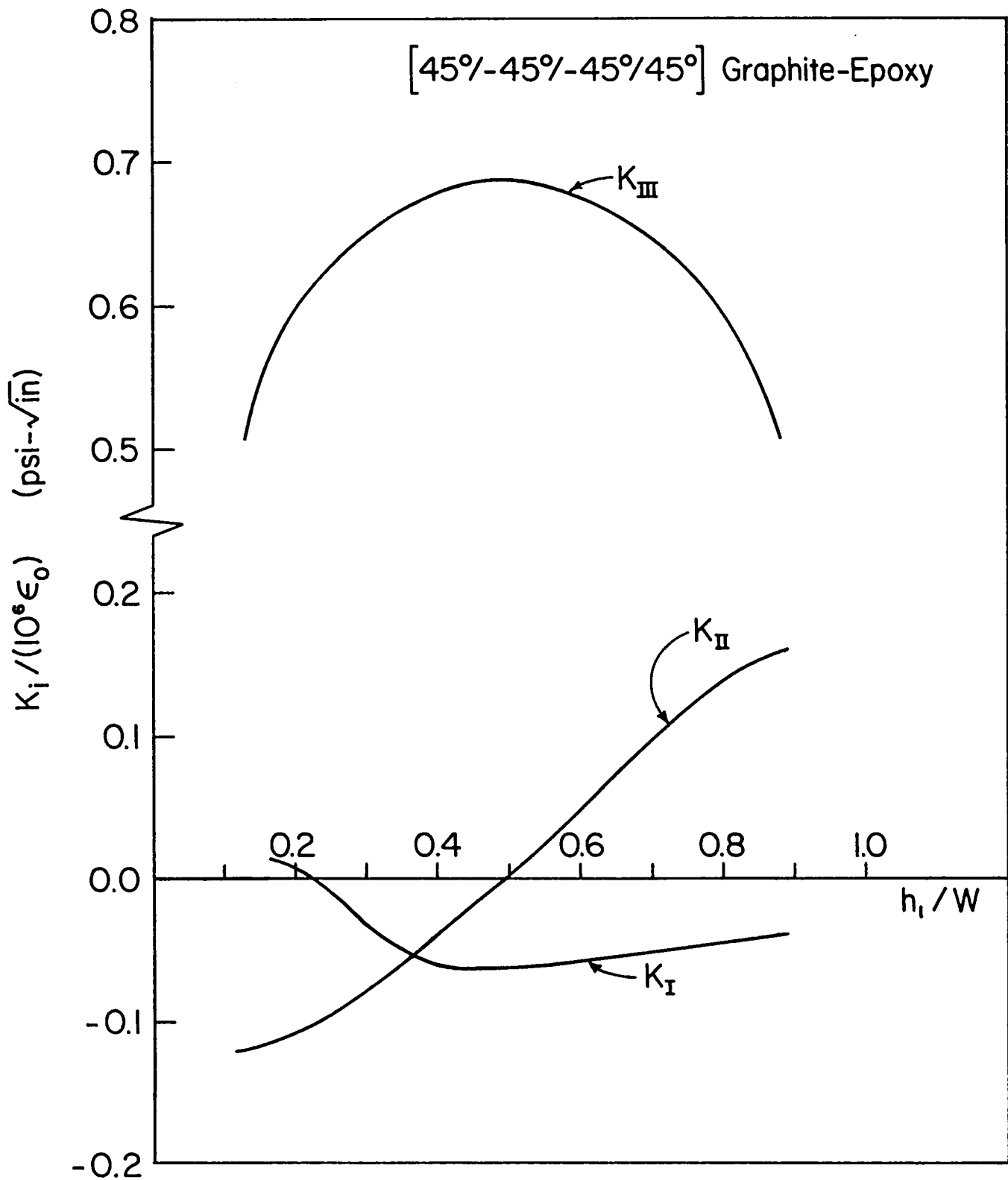
Fig. 8 Influence of Ply Thickness h_1/W on Stress Intensity Factors for Delamination in [45°/-45°/-45°/45°] Graphite-Epoxy Subjected to Uniform Axial Strain \epsilon_z = \epsilon_0 ( h_1 + h_2 = W = 0.5 in., 2b/W = 8 , a = 0.25 in.).
