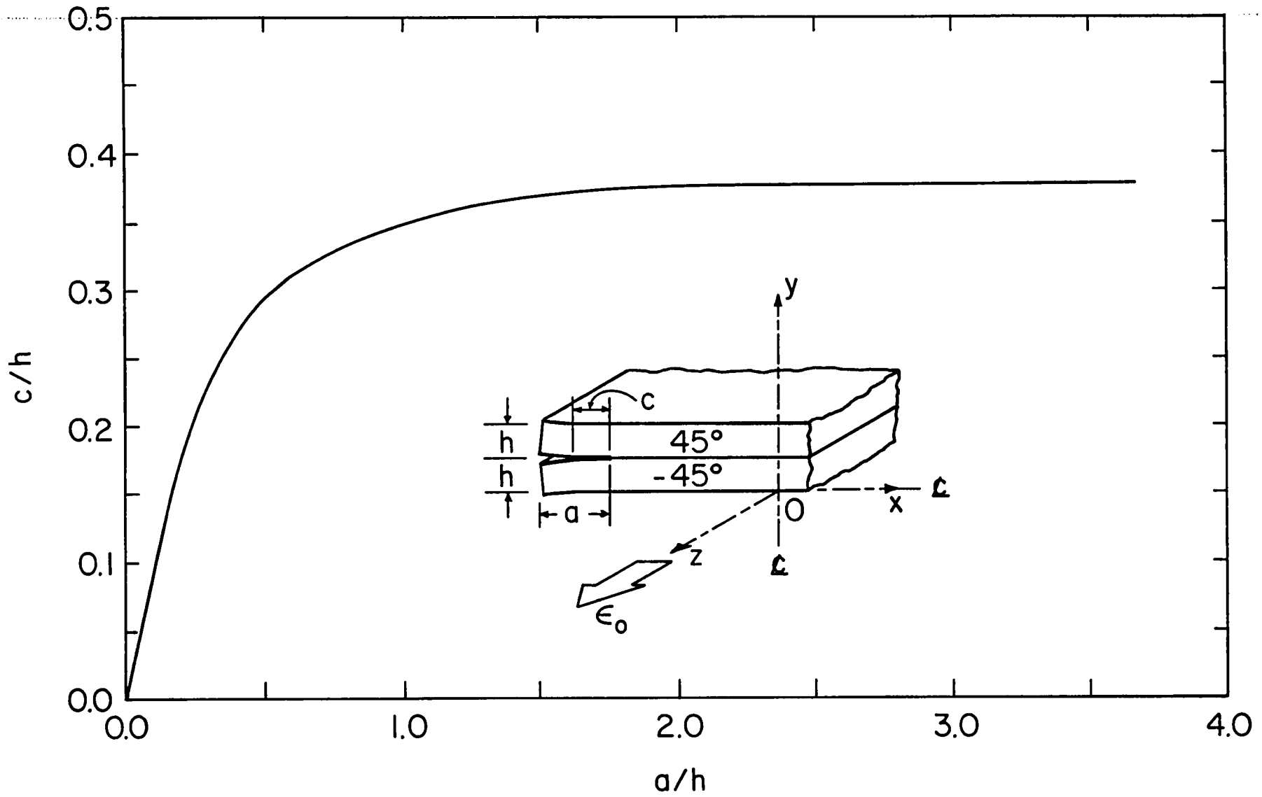
Fig. 11 Crack-Tip Closure Length c/h as a Function of Delamination Size a/h in [45^\circ/-45^\circ/-45^\circ/45^\circ] Graphite-Epoxy Subjected to Uniform Axial Strain \epsilon_z = \epsilon_0 ( h_1 = h_2 = h = 0.25 in., b/h = 8 , a = 0.25 in.).
