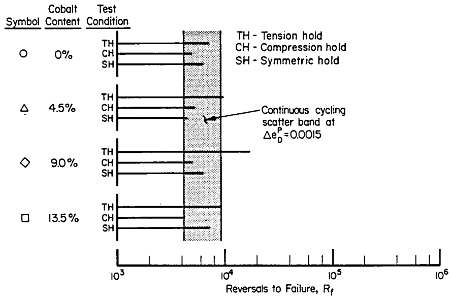
(e) Comparison of fatigue resistances as a function of cobalt content and strain history at \Delta e_D^P = 0.0015
