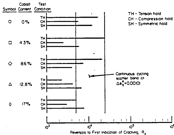
c. for Wrought U 700 at 760 C at \Delta\epsilon_p^p = 0.00101
