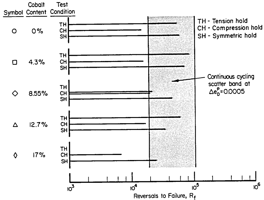
(f) Comparison of fatigue resistances as a function of cobalt content and strain history at \Delta e_D^p = 0.0005
