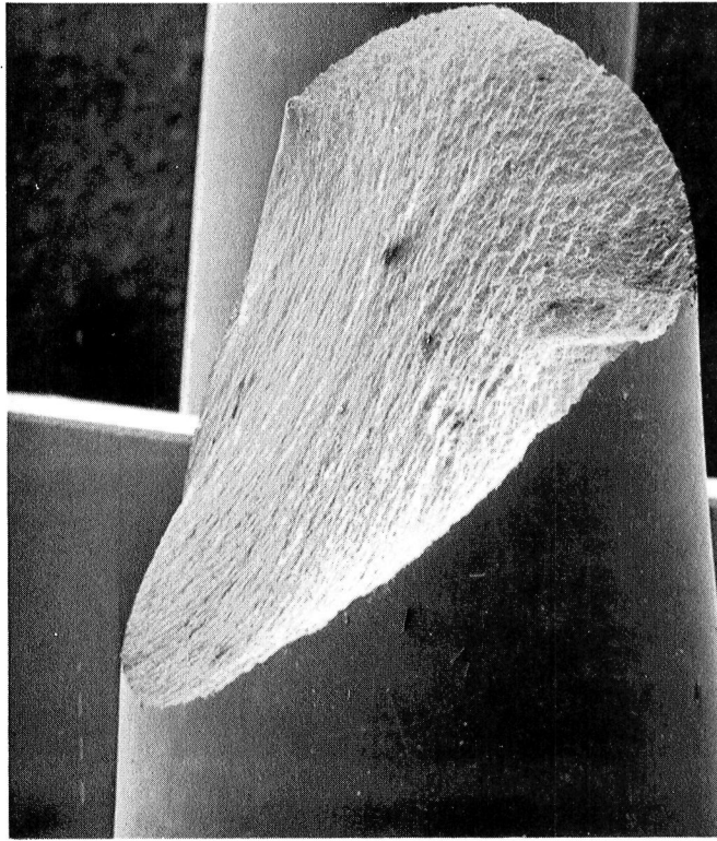
(a) Macroview of specimen D5-1947-1D-2; 0% Co alloy under tension hold cycling
