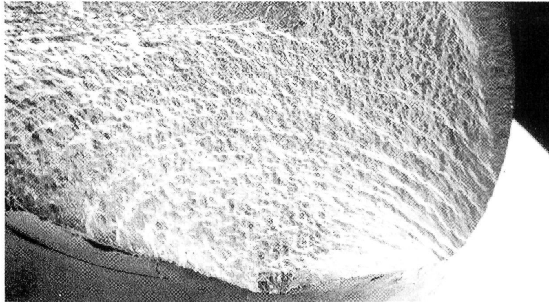
(b) Overview of fracture at origin in specimen D5-1949-1A-1; 9% Co alloy under continuous cycling
