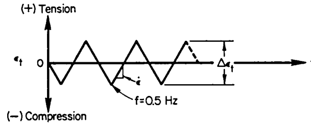
(a) Fully reversed strain-cycling wave form
