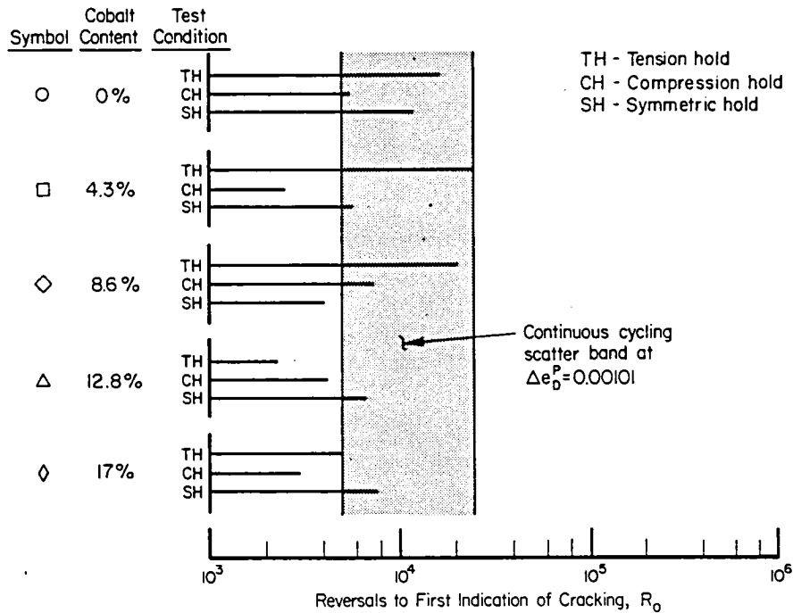
(f) Comparison of fatigue resistances as a function of cobalt content and strain history at \Delta\epsilon_D^P = 0.00101
