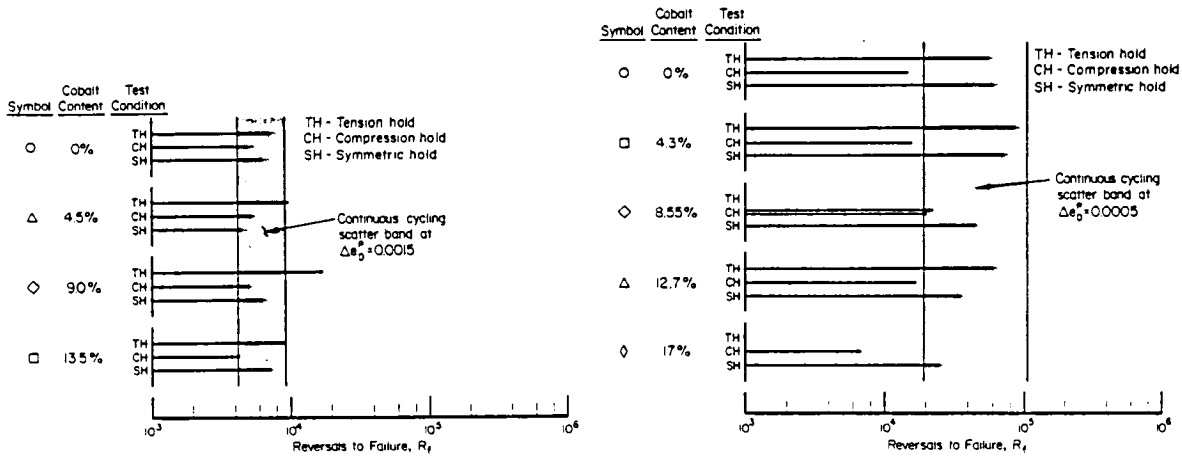
b. for PM U 700 at 760 C at \Delta\epsilon_p^p = 0.0005
