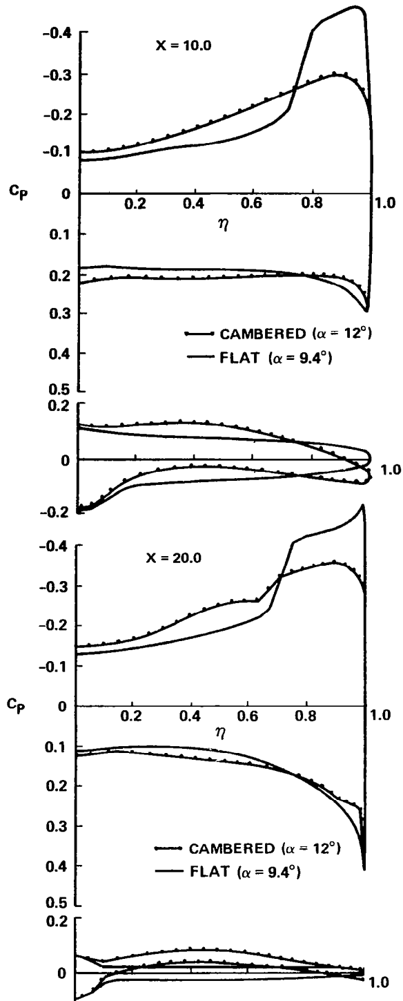
Figure 28. - Comparison of the flat and cambered wing shapes and predicted pressures at M = 1.62 and C_L = 0.40 .
