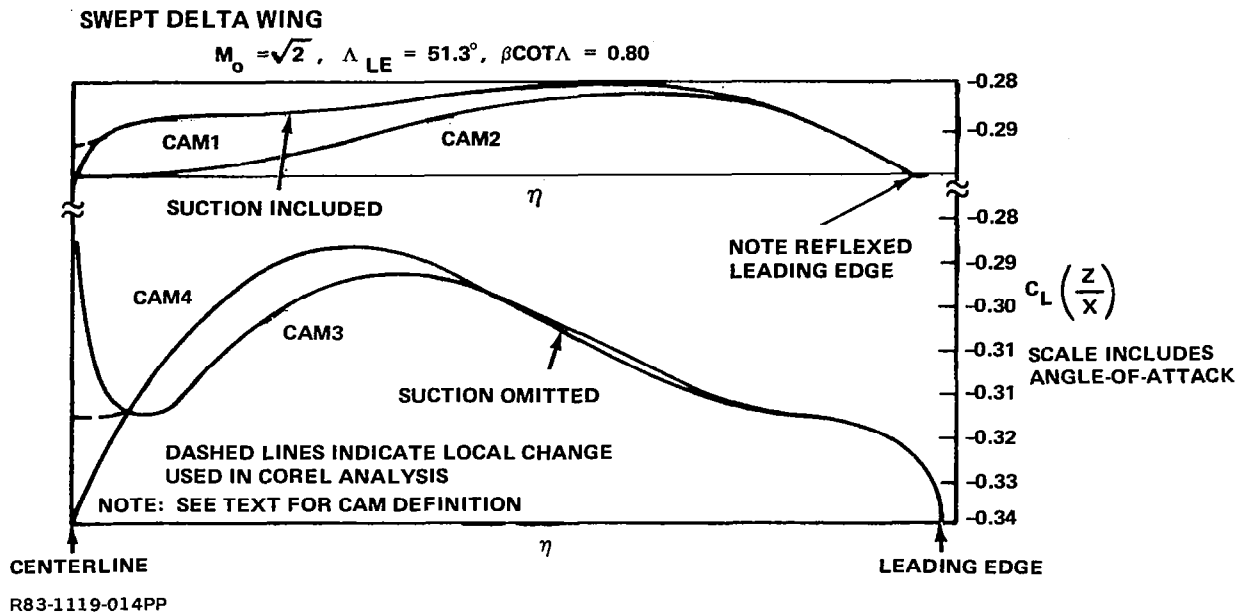
Figure 14. - Linear theory minimum drag spanwise camber shapes found by S.H. Tsien (ref. 16).
