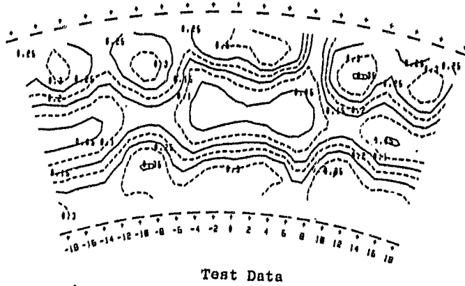
CONFIGURATION 6 OPPOSED-STAGED DILUTION INTO UNIFORM CROSSFLOW NR=10 1.25 INCHES DOWNSTREAM OF SECONDARY INJECTION POINT
