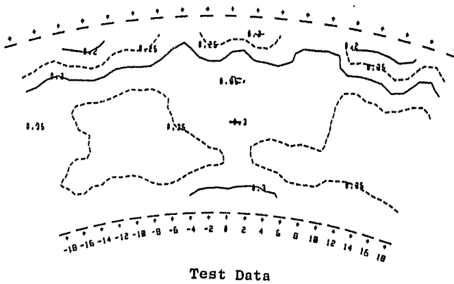
CONFIGURATION 7 OPPOSED-STAGED DILUTION INTO UNIFORM CROSSFLOW NR=50 1.25 INCHES DOWNSTREAM OF SECONDARY INJECTION POINT
