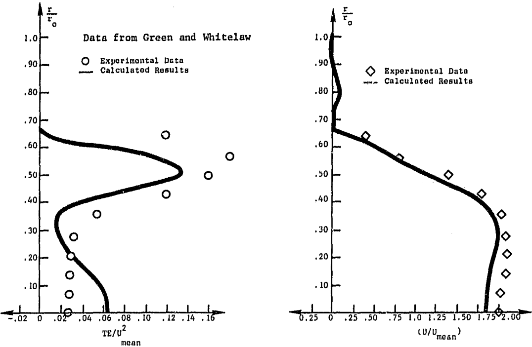
Figure 19. Radial Profile of Turbulence Kinetic Energy and Mean Axial Velocity at x/r_0 = 2.77 .
