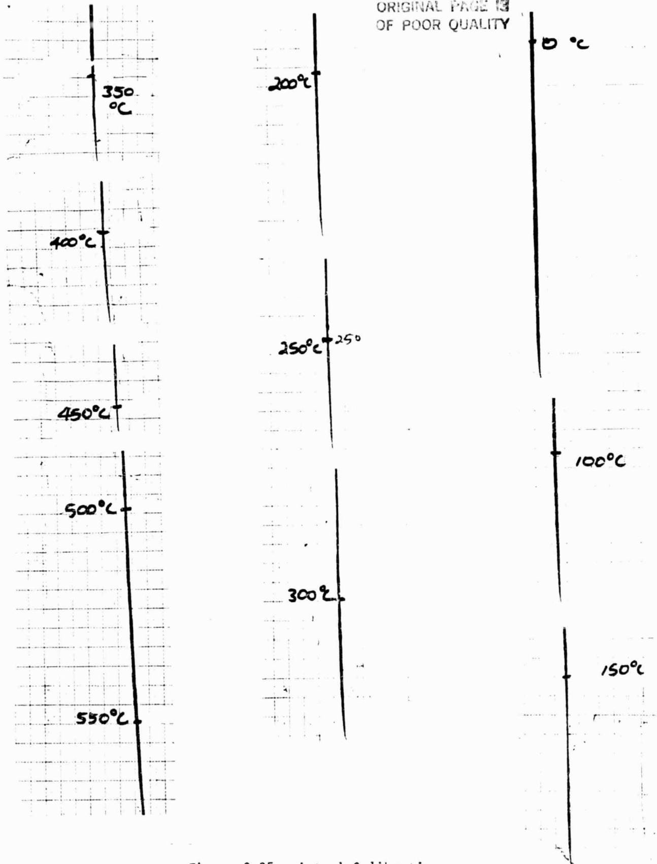
Figure C-25 - Actual Calibration Strips for the Temperature System
