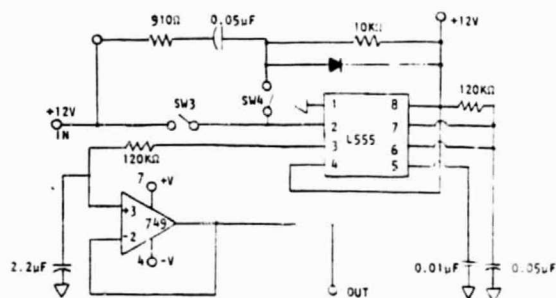
Figure C-4 - Second Rpm Circuit Diagram
