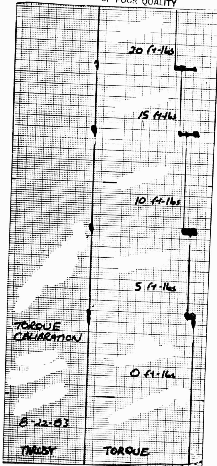
Figure C-17 - Actual Calibration Strips for the Torque System.
