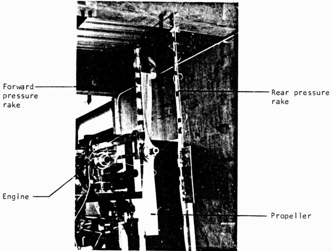
Figure E2 - Photograph of the \Delta P System
