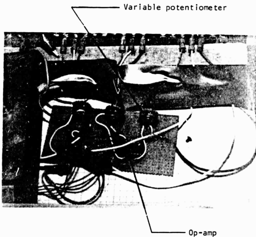
Figure 2.4 - Amplifier System Used to Amplify Transducer Signal
