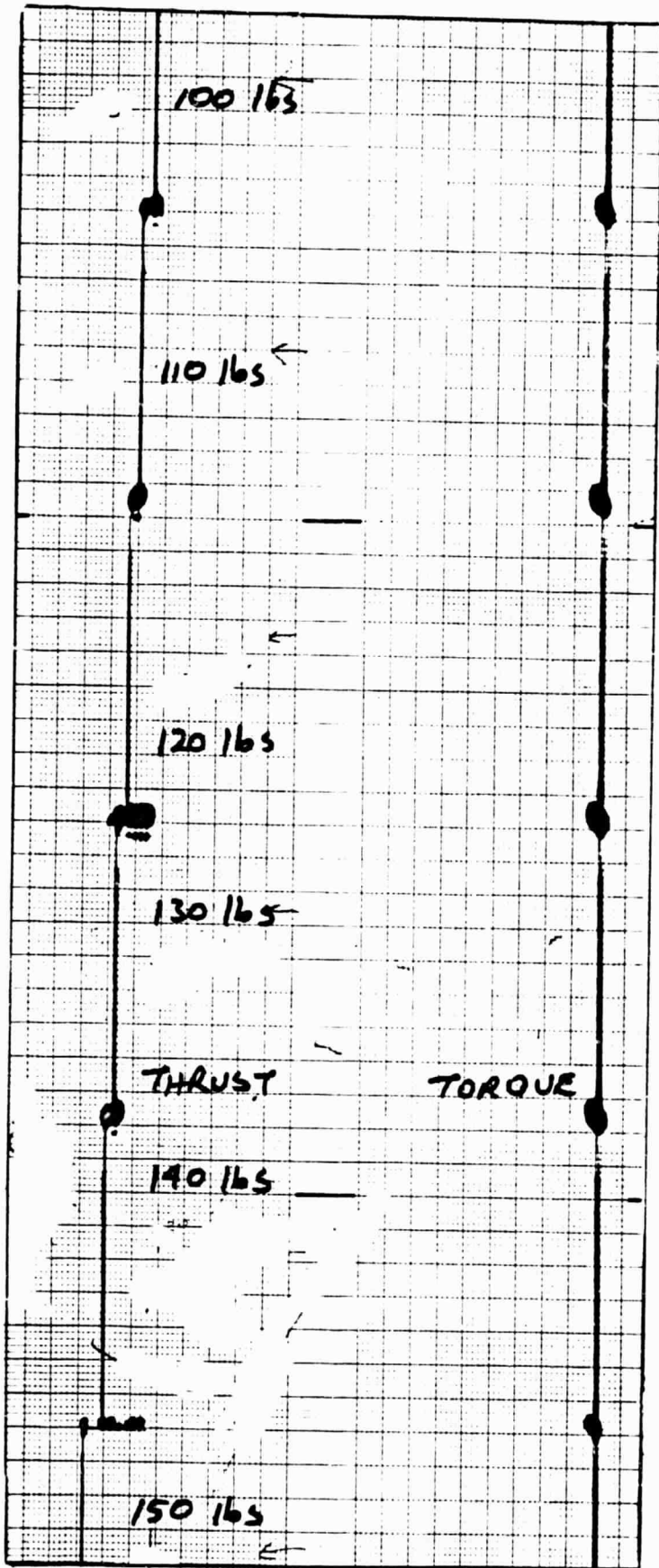
Figure C-12 - Actual Calibration Strips for the Thrust System.
