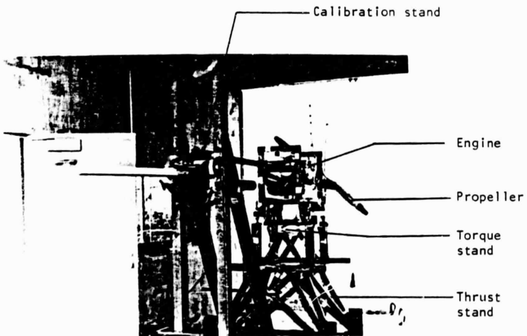
Figure C-10 - Photograph of the Thrust Calibration Stand
