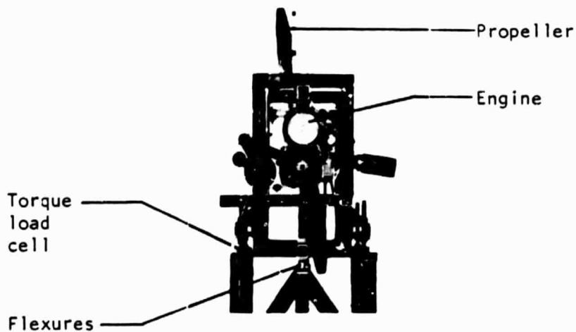
Figure 2.6 - Torque System
