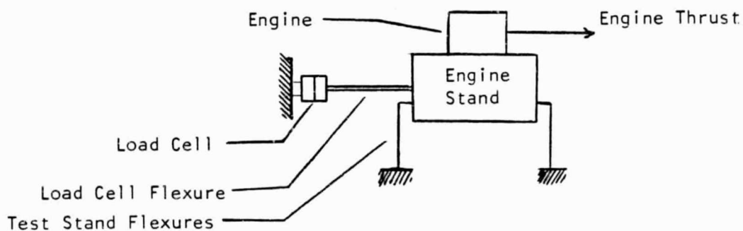
Figure C-7 - Schematic of the method for obtaining thrust
