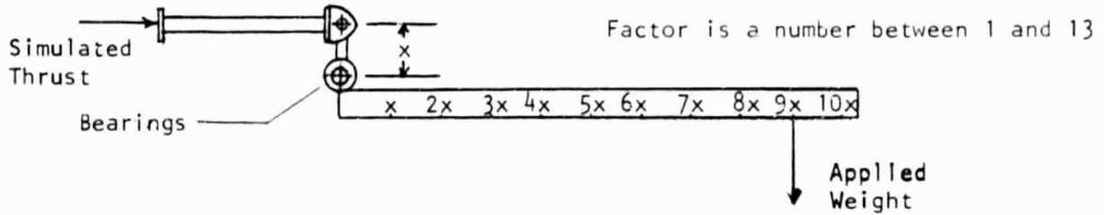
Figure B3 - Schematic of the Operation of the Thrust Calibration Stand
