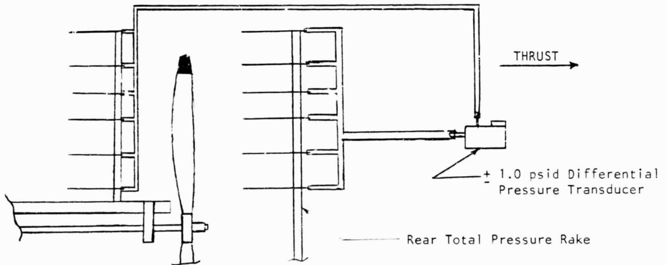
Figure E1 - Schematic of the \Delta P measuring system
