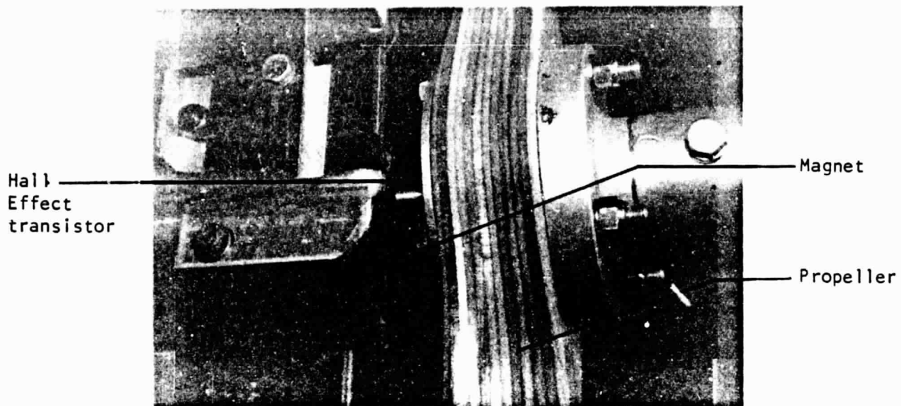
Figure 2.9 - Close-Up of the Hall Effect Transistor
