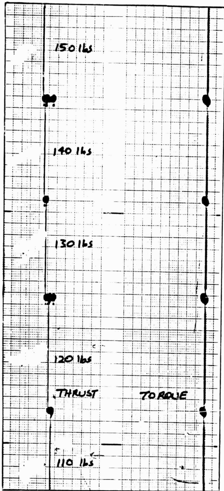
Figure C-12 - Actual Calibration Strips for the Thrust System.
