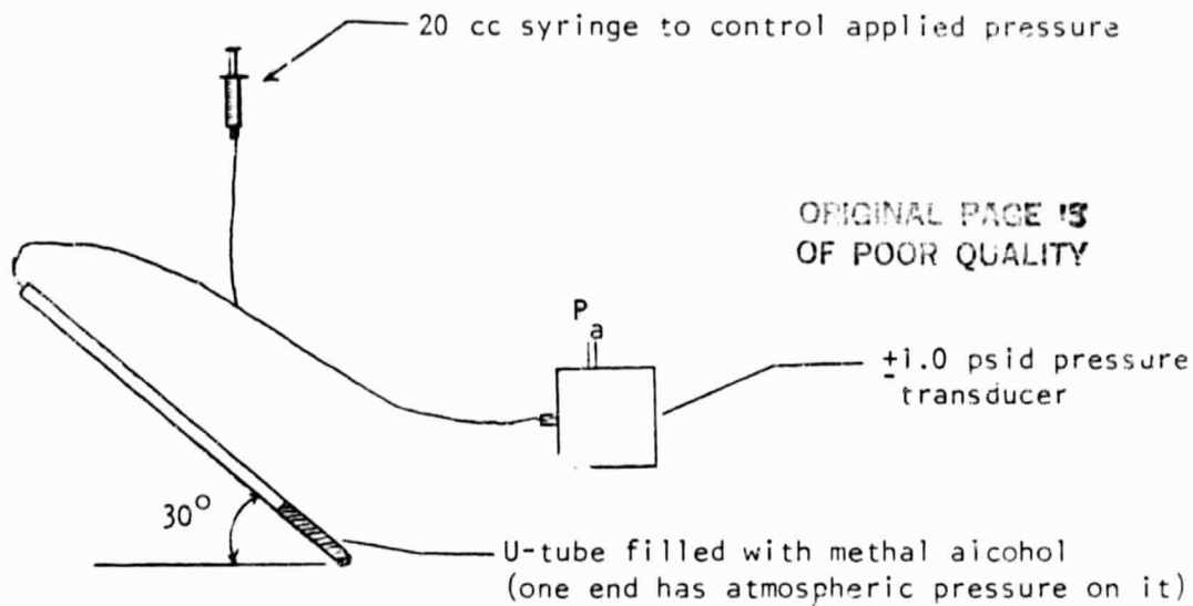
Figure C-21 - Schematic of the \Delta P Calibration Device
