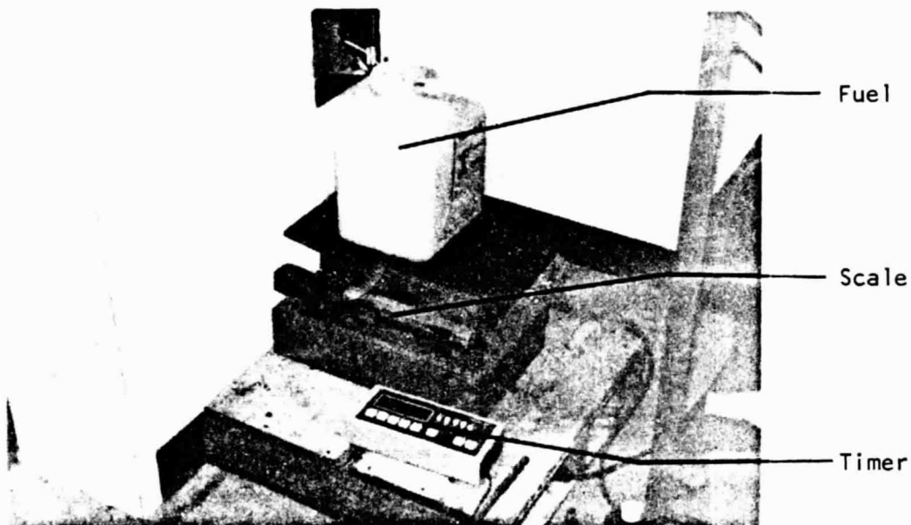
Figure 2.15 - Fuel Flow System Set-Up Including Scale and Timer
