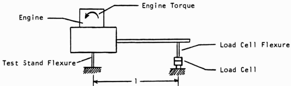
Figure C1 - Schematic for Obtaining Torque
