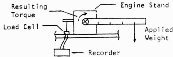
Figure B-2 - Schematic of the Torque Calibration Stand
