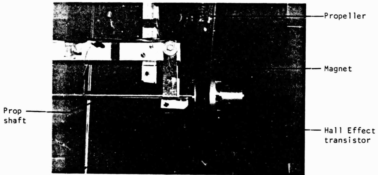
Figure 2.8 - RPM Measurement System
