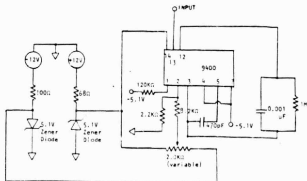
Figure C-2 - First Propeller RPM Circuit
