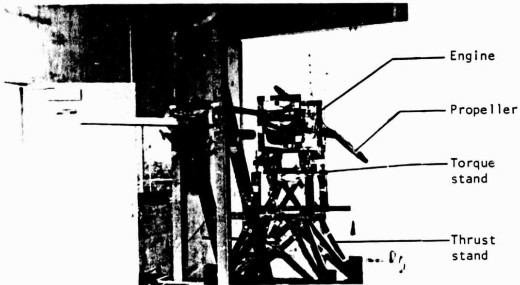
Figure 2.1 - Static Test Stand at the Mel Harned Propulsion Laboratory. (Note: Thrust calibration stand is installed in this figure.)
