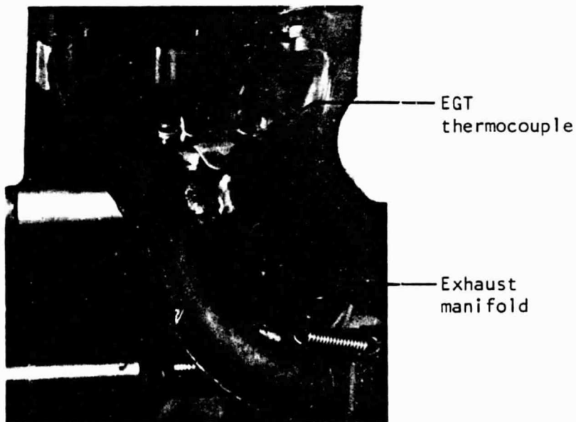
Figure 2.13 - Exhaust Gas Temperature Thermocouple Place in Exhaust Gas Manifold
