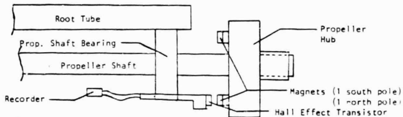
Figure C-1 - Positioning of the Hall Effect Transistor
