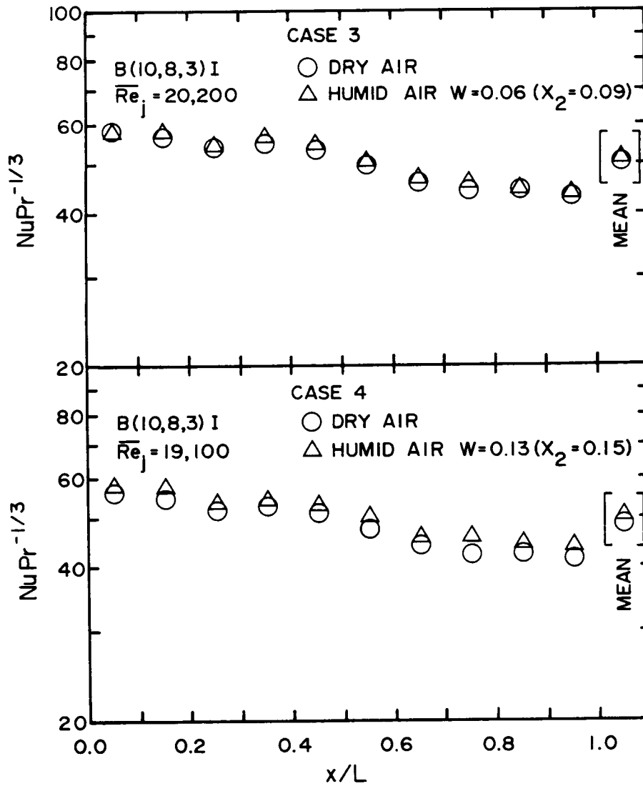
Fig. 5.2 NuPr^{-1/3} for Dry versus Humid Air for B(10,8,3)I Geometry
