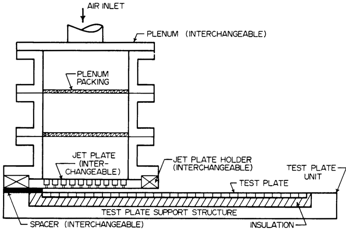
CHORDWISE VIEW
