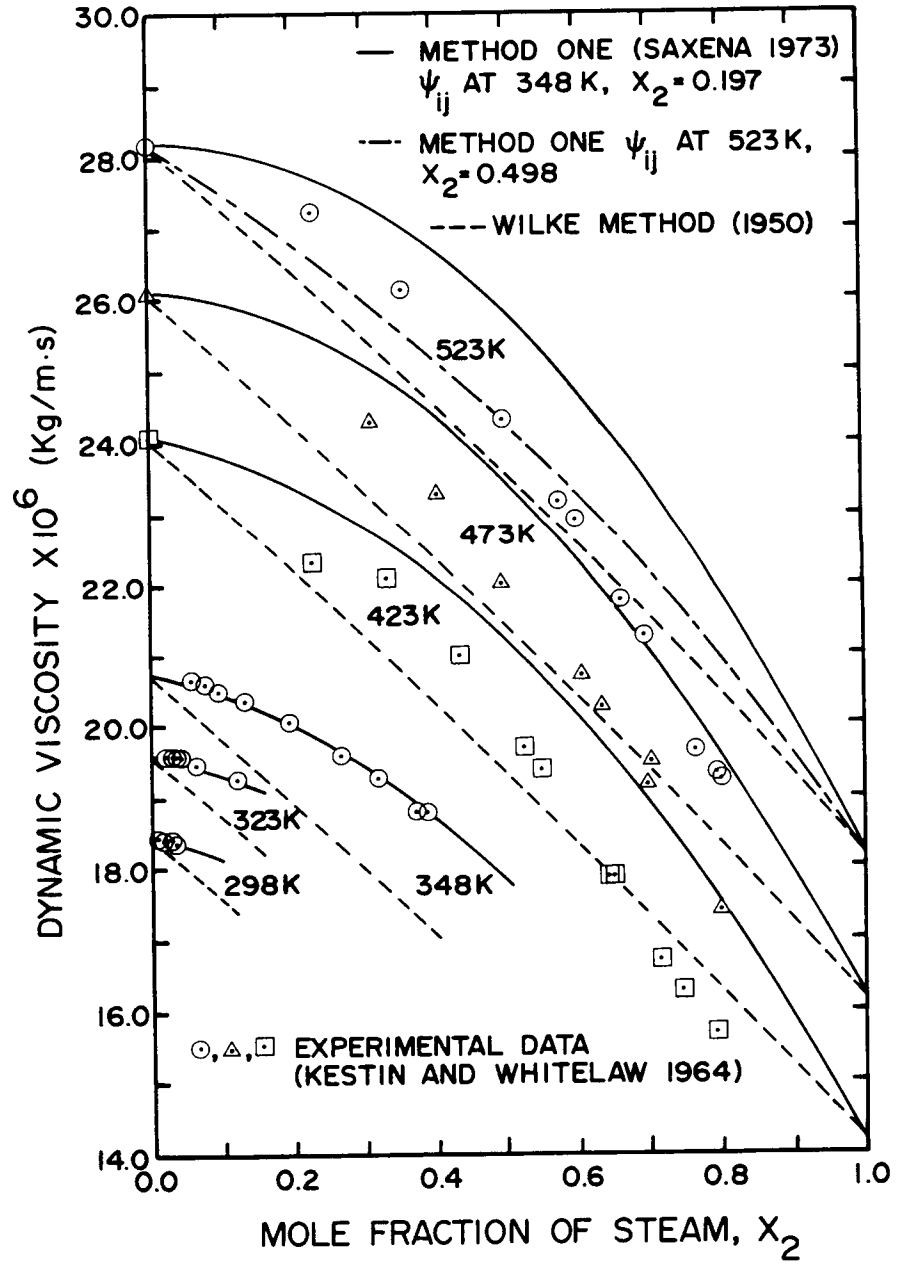
Fig. 2.1 Dynamic Viscosity of Humid Air at Several Temperature Levels
