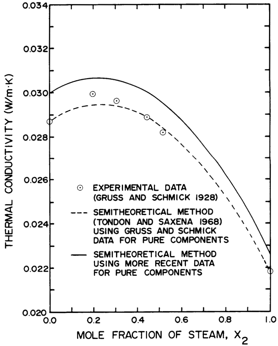
Fig. 2.2 Thermal Conductivity of Humid Air at 353 K
