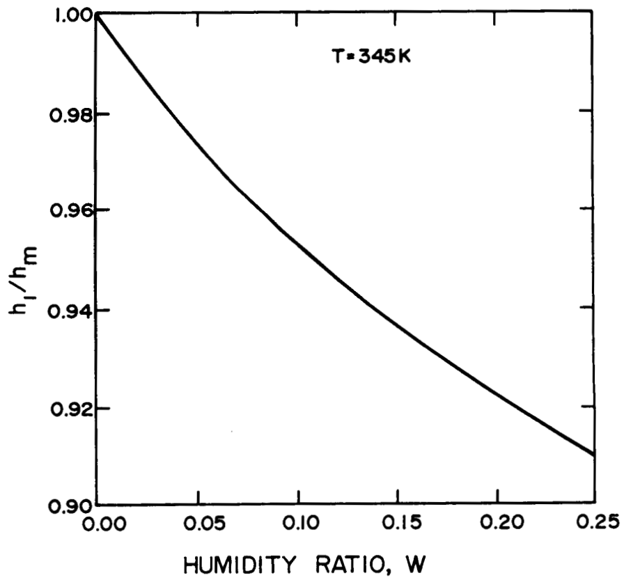
Fig. 5.4 Effect of Humidity Ratio on Heat Transfer Coefficient
