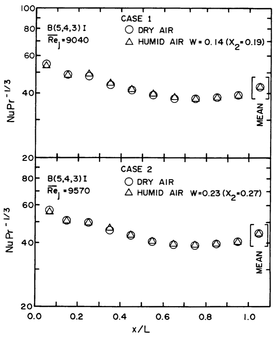
Fig. 5.1 NuPr^{-1/3} for Dry versus Humid Air for B(5,4,3)I Geometry
