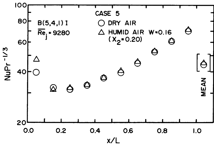
Fig. 5.3 NuPr^{-1/3} for Dry versus Humid Air for B(5,4,1)I Geometry
