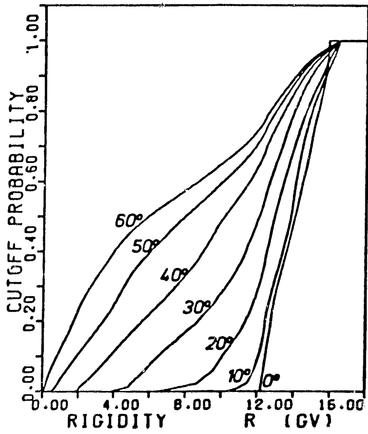
Figure A-8. Geomagnetic Shielding Factors at 223 km (Source: Reference A-4)
