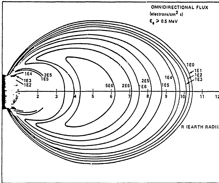
Figure A-3. Electron Distribution in the Earth's Field (Source: Reference A-2)
