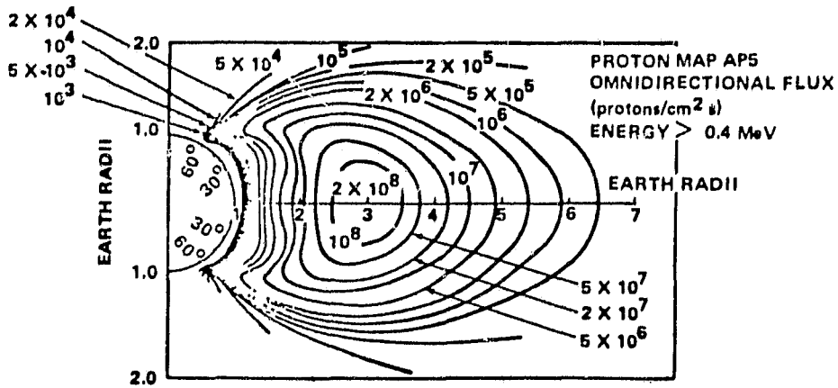
Figure A-4. Proton Distribution in the Earth's Field (Source: Reference A-2)
