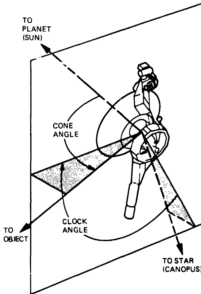
Fig. 3. Definition of cone and clock angles
