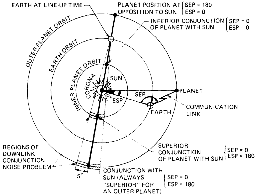
Fig. 6. Definition of opposition and conjunction events involving Sun, Earth, and planet
